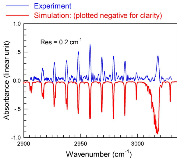
Fig. 5. Comparison between the measured and simulated absorption spectrum (fitting parameters: 0.65% methane at 1 atm; 20 cm cell; resolution = 0.2 cm -1 ).
