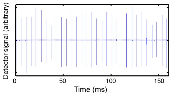
Fig. 2. Time-domain interferogram ( \Delta f = 96 Hz). One of the mid-IR pulse sequences operated in a double-pulse mode.
