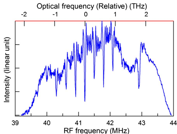
Fig. 3. Fourier-transform spectrum expressed in the RF (lower axis) and optical (upper axis) domains.
