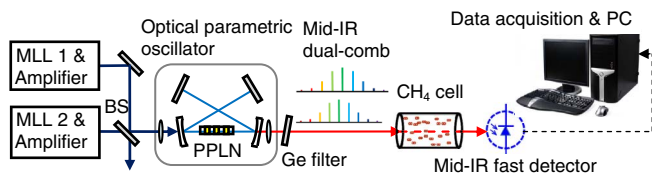
Fig. 1. Layout of the mid-IR dual-comb spectrometer. MLL, mode-locked laser; BS, beam splitter; PPLN, periodically poled lithium niobate.
