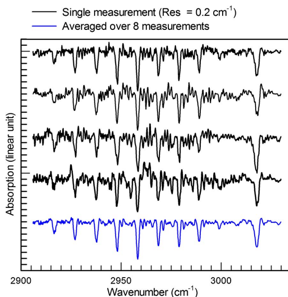
Fig. 4. Normalized methane absorption spectra for single measurements (top 4 traces, black) and an averaged spectrum (bottom trace, blue).
