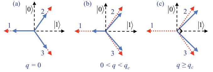
FIG. 1. (Color online) The optimal measurement operators we should aim for when distinguishing between the three symmetric quantum states in Eq. (12), when the final detection is imperfect so that outcome 1 is misidentified as outcome 2 or 3 with probability q . The states to be distinguished are shown using dotted arrows (red), and the measurement operators are (un-normalized) projectors onto the states indicated by solid arrows (blue). The basis states |0\rangle and |1\rangle are indicated with dashed arrows (black). In (a), the detection is perfect, and the measurement operators are proportional to projectors onto the states themselves. In (b), 0 < q < q_c , and, in (c), q \geq q_c . It pays to concentrate more on the states we can identify more reliably.
