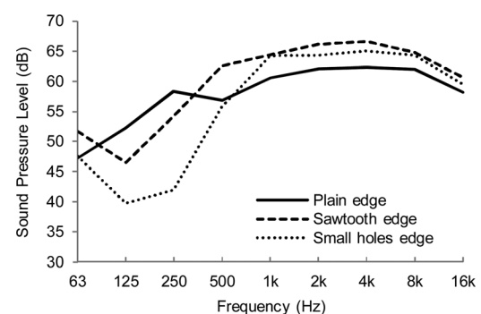
FIG. 5. Impact of waterfall's edge design on sound spectra (waterfall of 1 m width and 1 m height, with a flow rate of 30 l/min).
