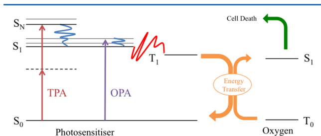
Figure 1. Modified Jablonski diagram indicating the energy flow from the excited photosensitizer species, achieved through either one- or two-photon absorption, leading to the generation of singlet oxygen, and subsequent cell death. The dashed horizontal line represents a virtual state.
