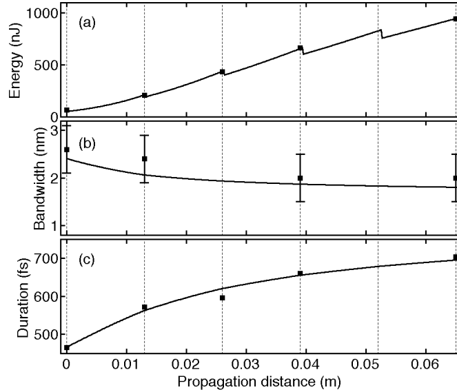
Fig. 3. Numerical modelling results (solid lines) fitted to experimentally measured pulse parameters (symbols) by adjusting E_{sat} , g_0 and \Delta\lambda_g . Propagation between neighboring dashed vertical lines represents one pass through the 13-mm-long Yb:YAG crystal. The error bars in (b) represent the \pm 0.5 nm accuracy of the spectrometer used to record the pulse spectra.
