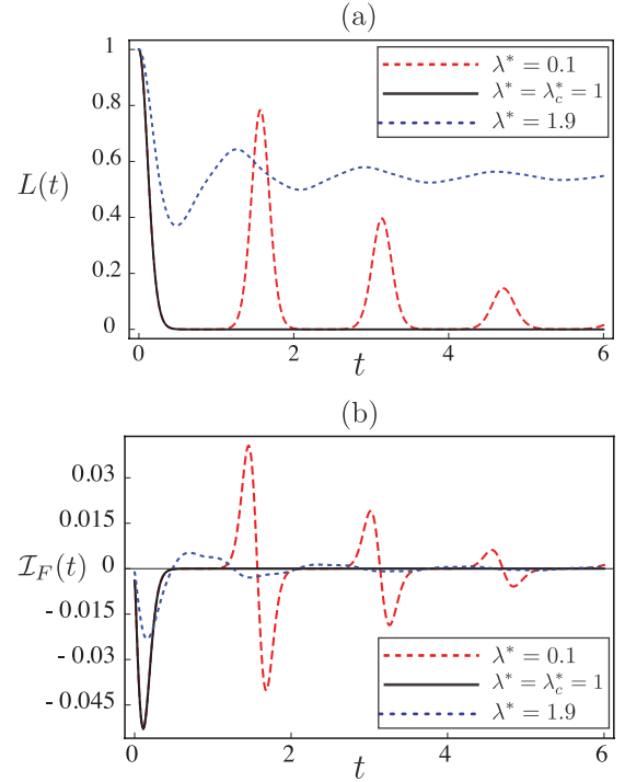
FIG. 1. (Color online) (a) The Loschmidt echo and (b) the Fisher information flow induced by the coupling of a central spin to the transverse Ising model consisting of N = 4000 spins for three different values of the transverse field. We choose J = 1 and \delta = 0.01 . The sensitivity to the critical point \lambda_c^* = 1 is dramatic. Note that in (a), the solid black curve and the dashed red curve overlap for initial times.
