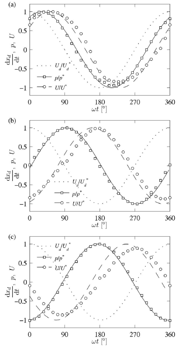
FIG. 1. Phase-locked cavity pressure p and jet velocity U for (a) \omega = 0.26\omega_0 , (b) \omega = \omega_0 , and (c) \omega = 2.6\omega_0 .
