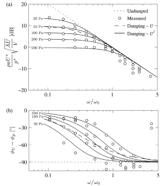
FIG. 2. Experimental validation of the pressure-velocity relationship using the proposed model, with linear and nonlinear damping described by Eqs. (6) and (8).
