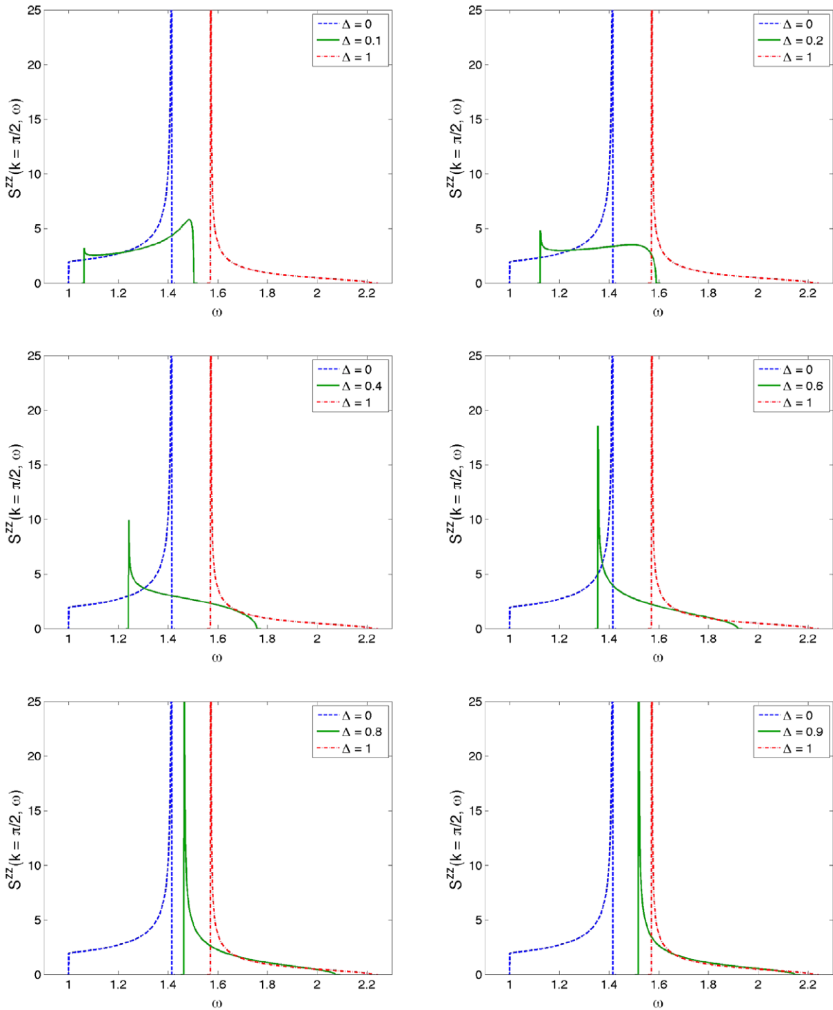
Figure 4. Fixed momentum cuts at k = \pi/2 of the two-spinon part of the longitudinal structure factor of the infinite Heisenberg chain, for different values of the anisotropy parameter \Delta . The \Delta = 0 and 1 limits are displayed in all plots for comparison.
