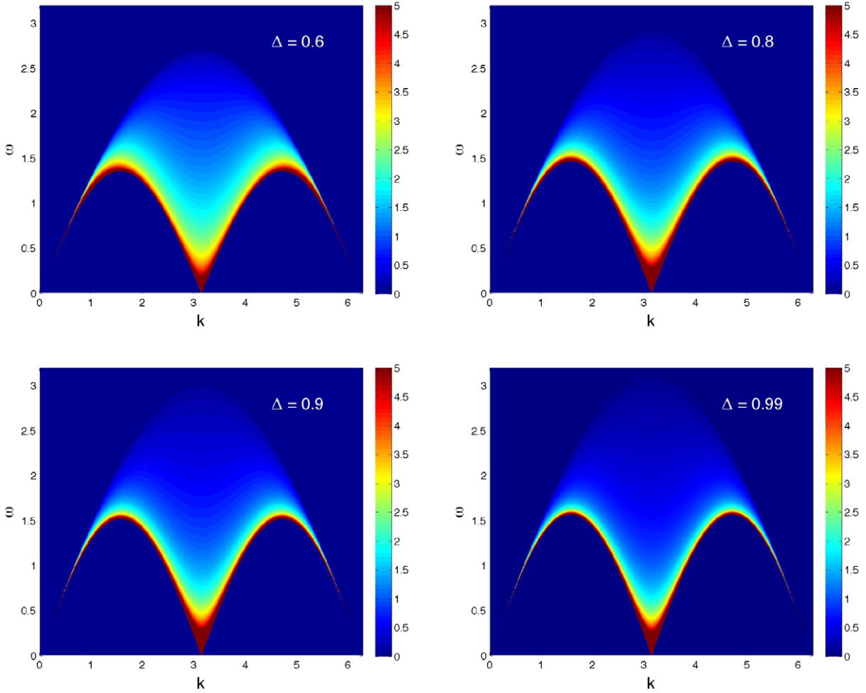
Figure 2. Two-spinon part of the longitudinal structure factor of the infinite Heisenberg chain, for different values of the anisotropy parameter \Delta (see also figure 2). Increasing the anisotropy shifts the weight progressively towards the lower boundary. The lower boundary becomes increasingly sharp as the \Delta \rightarrow 1 limit is approached.
