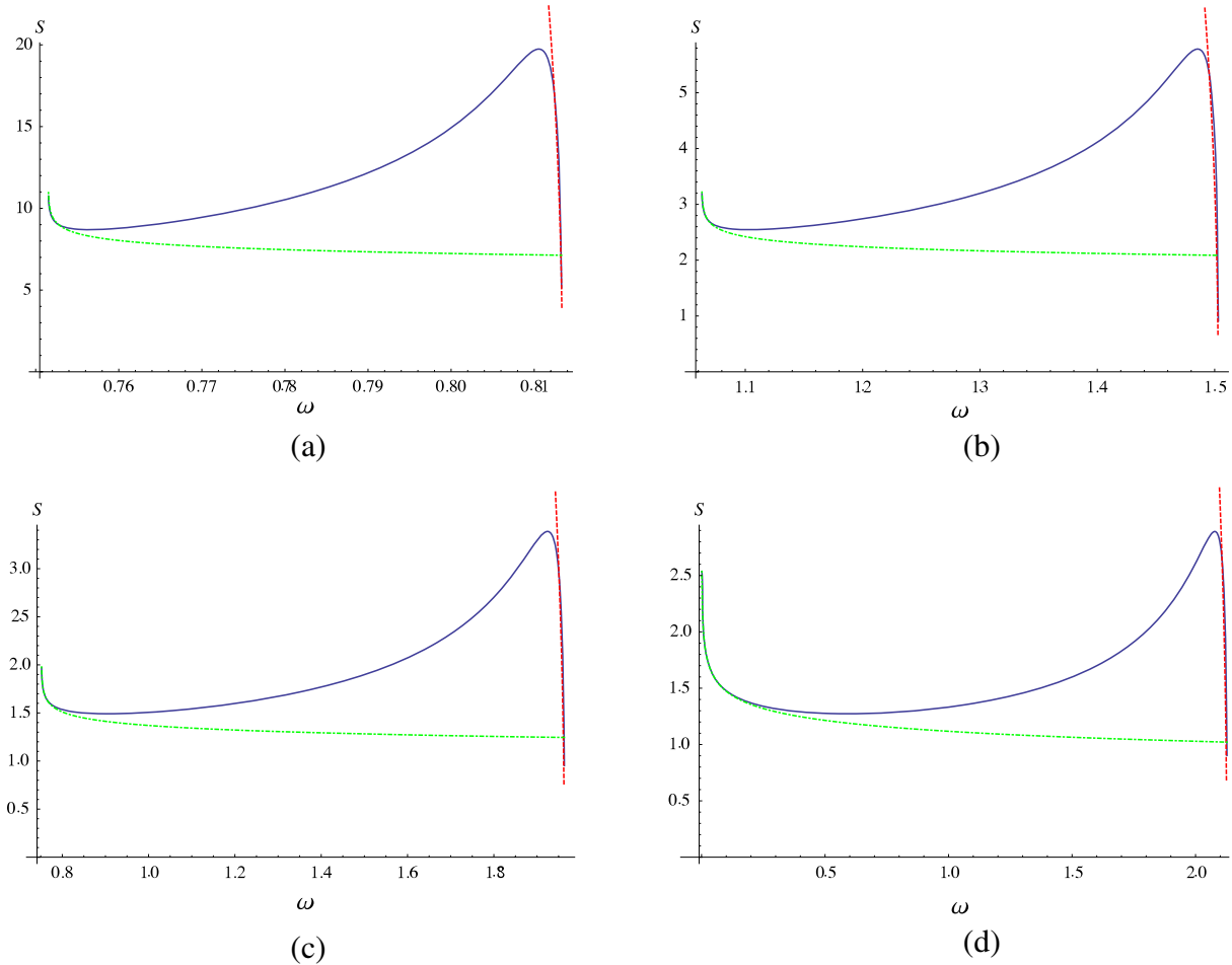
Figure 8. Threshold behaviour for \Delta = 0.1 . The solid line is the numerical evaluation of S_2^{zz} , while the dashed and dotted lines indicate the upper and lower threshold behaviours, respectively, fitted using the second method (see main text). (a) k/2\pi = 0.125 , (b) k/2\pi = 0.25 , (c) k/2\pi = 0.375 and (d) k/2\pi = 0.5 .
