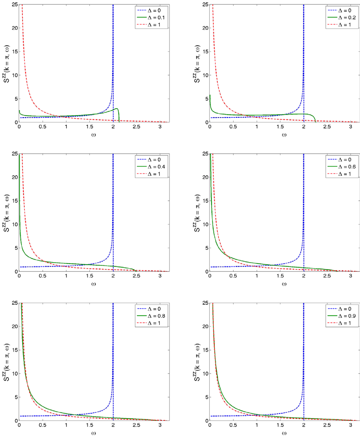
Figure 6. Fixed momentum cuts at k = \pi of the two-spinon part of the longitudinal structure factor of the infinite Heisenberg chain for different values of the anisotropy parameter \Delta . The \Delta = 0 and 1 limits are displayed in all plots for comparison.
