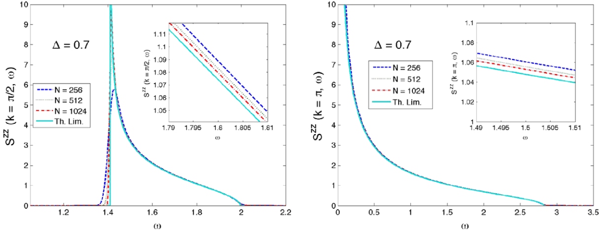
Figure 7. Comparison between the two-spinon longitudinal structure factor for \Delta = 0.7 and momentum k = \pi/2 (left) and k = \pi (right), in the thermodynamic limit (solid curve) and at finite size. The finite-size results are obtained by summing exactly over the set of N(N + 2)/8 two-spinon states at chain length N , and are plotted after Gaussian smoothing of the delta function contributions. See main text for more details.
