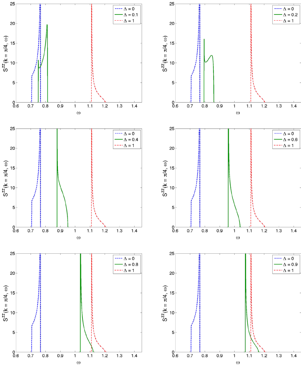
Figure 3. Fixed momentum cuts at k = \pi/4 of the two-spinon part of the longitudinal structure factor of the infinite Heisenberg chain for different values of the anisotropy parameter \Delta . The \Delta = 0 and 1 limits are displayed in all plots for comparison.
