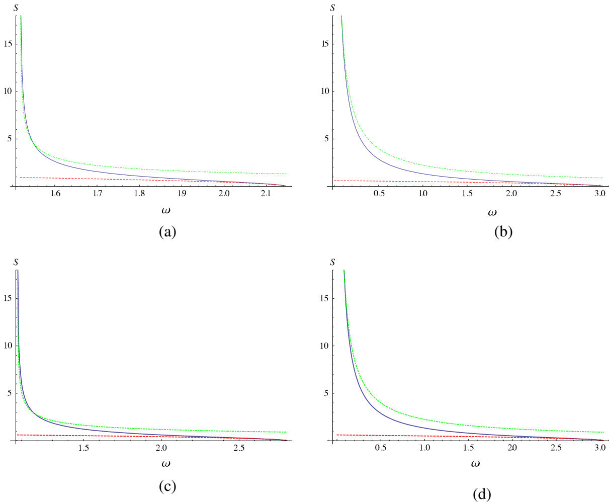
Figure 10. Threshold behaviour for \Delta = 0.9 . The solid line is the numerical evaluation of S_2^{zz} , while the dashed and dotted lines indicate the upper and lower threshold behaviours, respectively, fitted using the second method (see main text). (a) k/2\pi = 0.125 , (b) k/2\pi = 0.25 , (c) k/2\pi = 0.375 and (d) k/2\pi = 0.5 .
