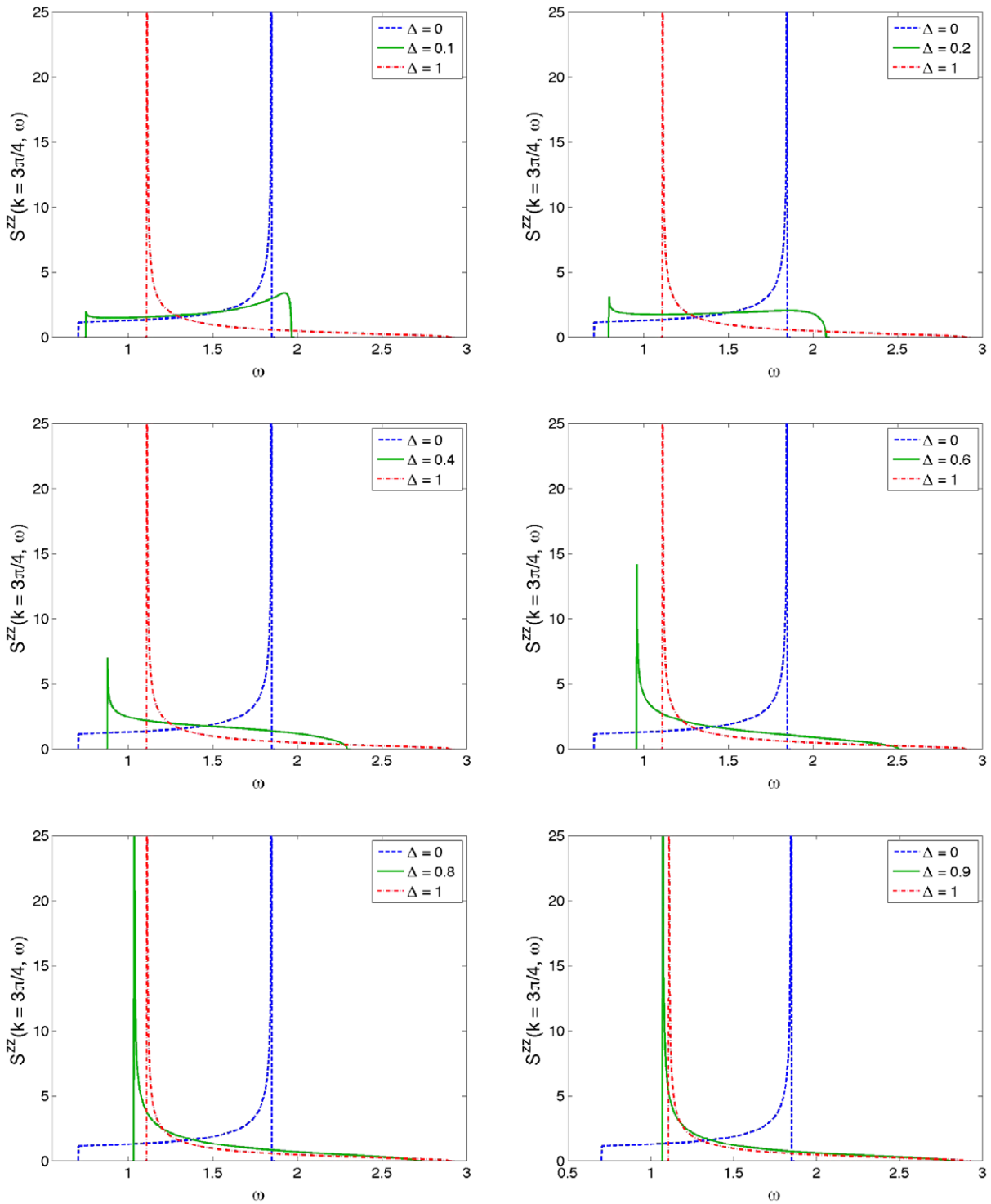
Figure 5. Fixed momentum cuts at k = 3\pi/4 of the two-spinon part of the longitudinal structure factor of the infinite Heisenberg chain for different values of the anisotropy parameter \Delta . The \Delta = 0 and 1 limits are displayed in all plots for comparison.
