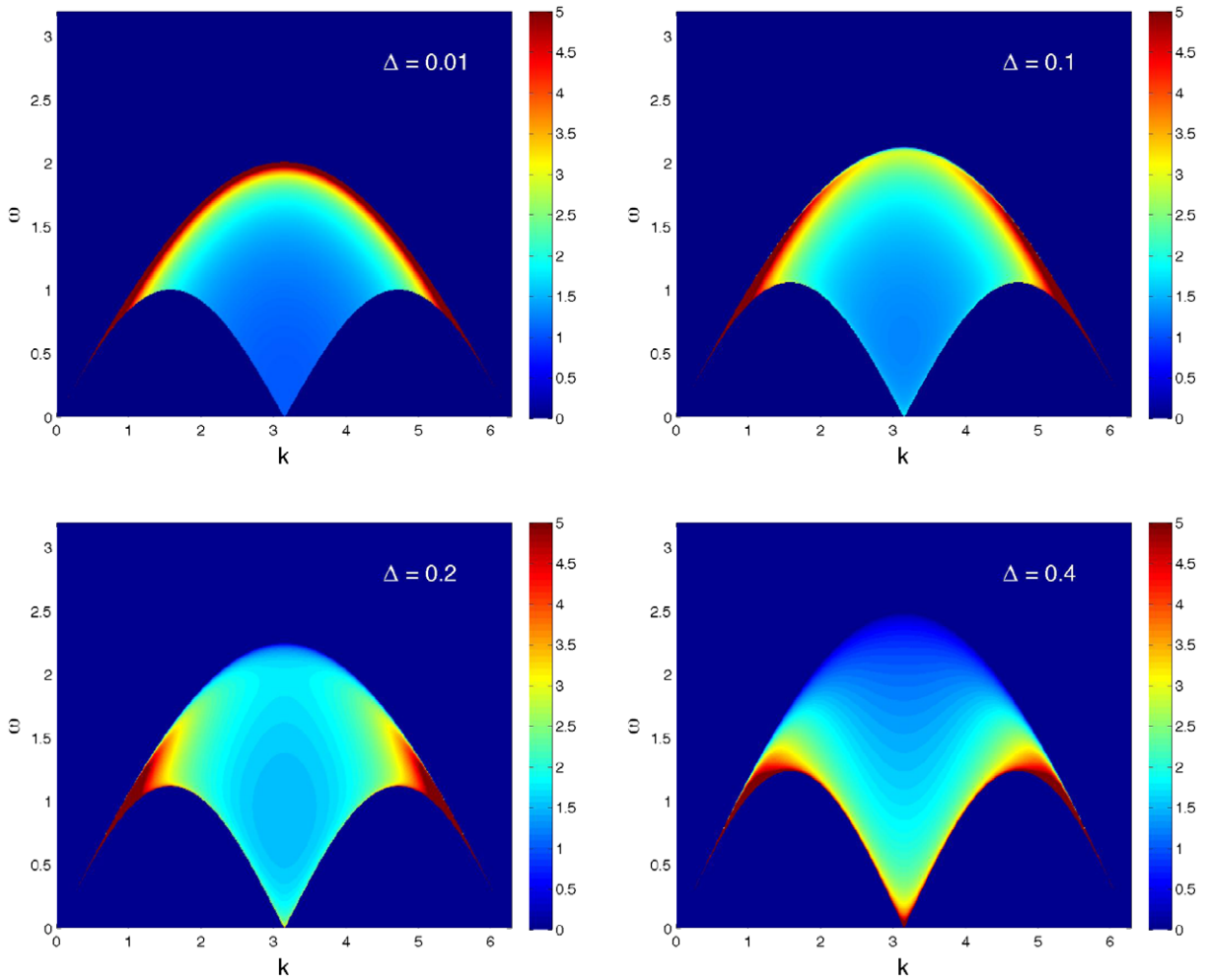
Figure 1. Two-spinon part of the longitudinal structure factor of the infinite Heisenberg chain, for different values of the anisotropy parameter \Delta (see also figure 2). For \Delta \rightarrow 0 , the correlation follows the density of states and has a square-root singularity at the upper threshold for all values of momenta.
