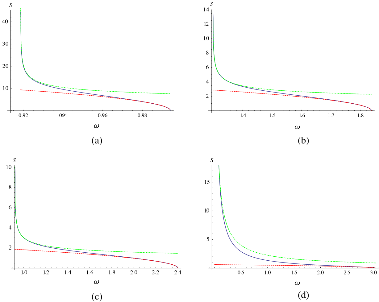
Figure 9. Threshold behaviour for \Delta = 0.5 . The solid line is the numerical evaluation of S_2^{zz} , while the dashed and dotted lines indicate the upper and lower threshold behaviours, respectively, fitted using the second method (see main text). (a) k/2\pi = 0.125 , (b) k/2\pi = 0.25 , (c) k/2\pi = 0.375 and (d) k/2\pi = 0.5 .
