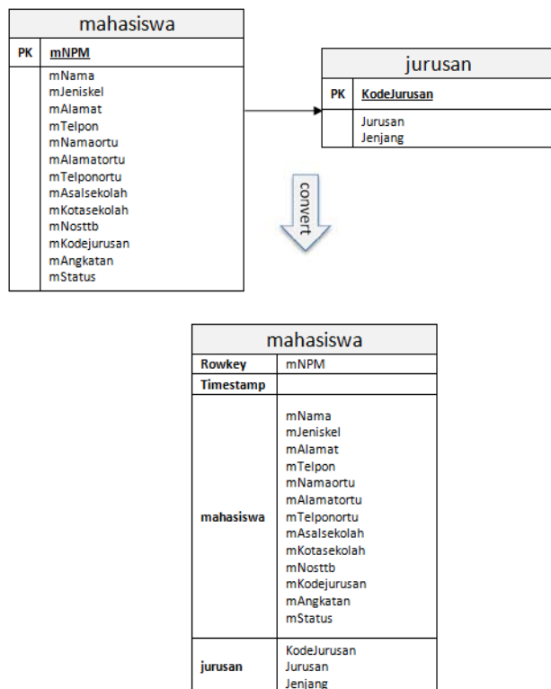
Fig. 2 Single nested scheme conversion designs for 'Mahasiswa' and 'Jurusan' Tables.
