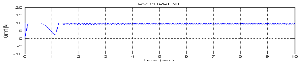
Figure 6. Output current waveform of PV
