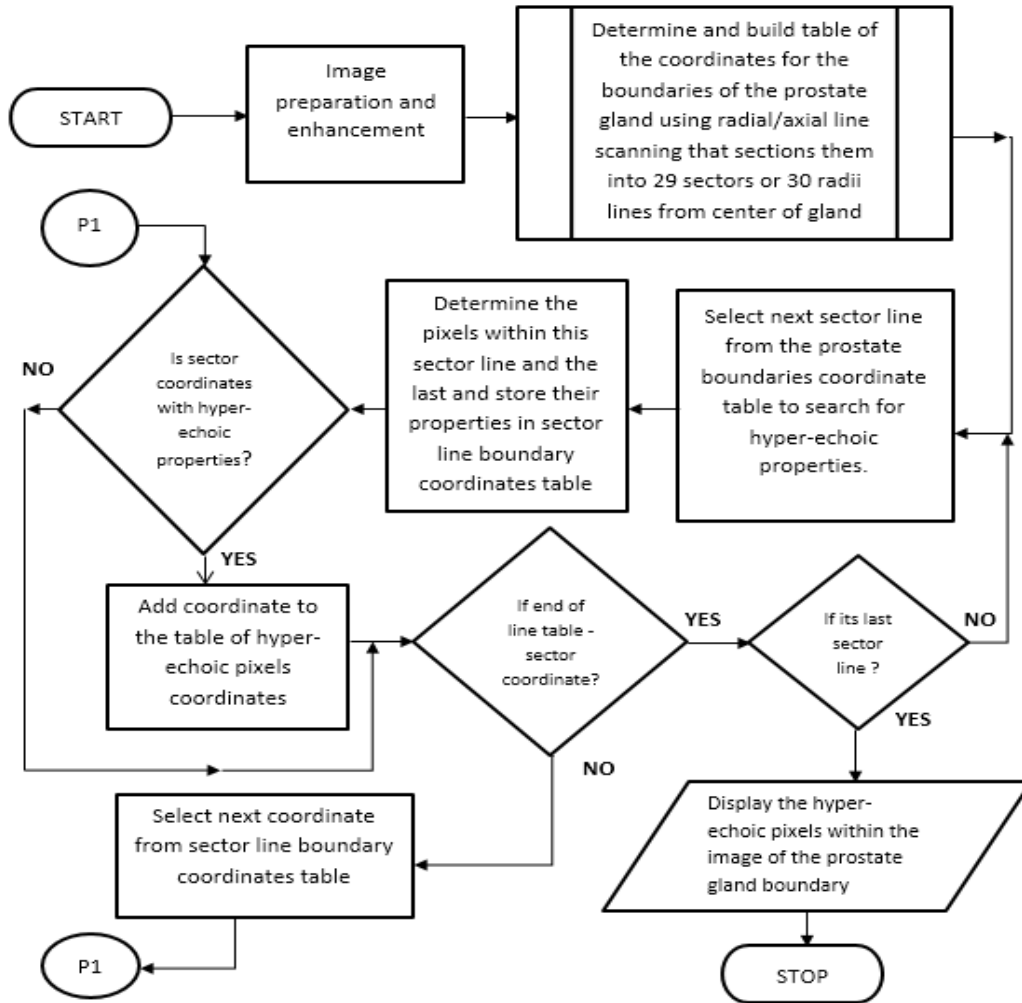
Figure 1. Flowchart of prostate cancer detection algorithm
