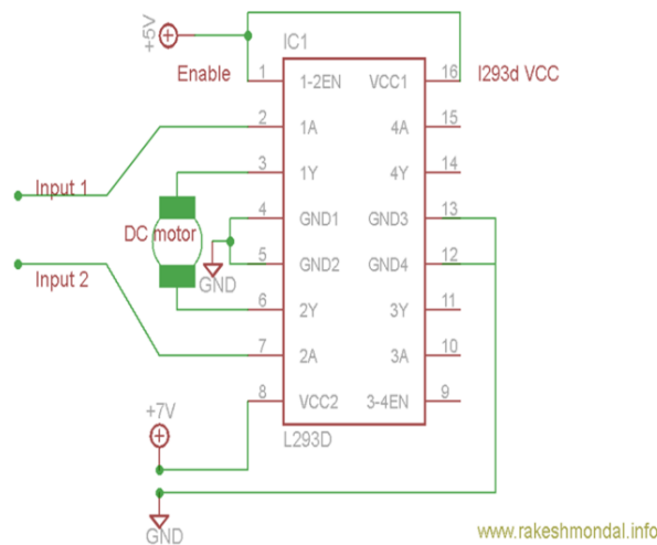
Figure 4. L293D motor driver circuit
