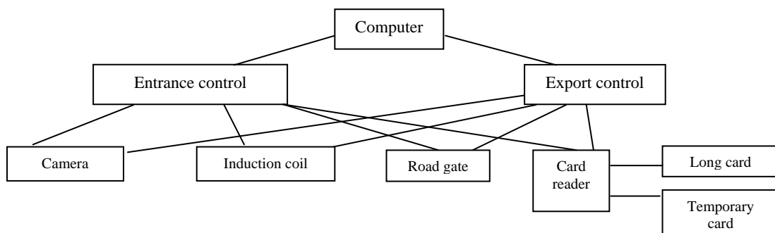
Figure 3. Hardware Design of City ETC System
