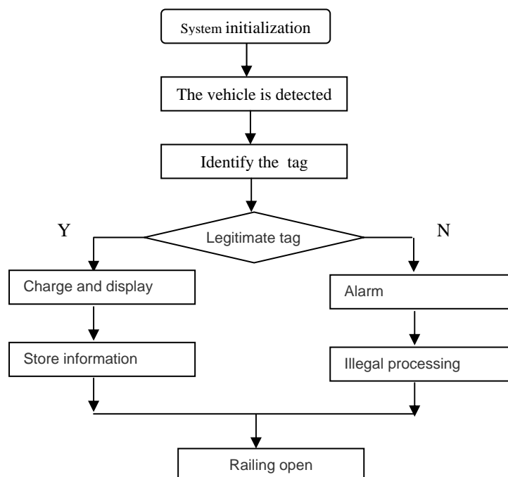
Figure 4. Workflow of ETC System
