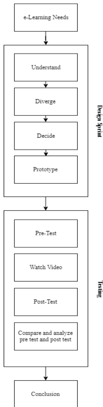
Gambar 5 Methodology
