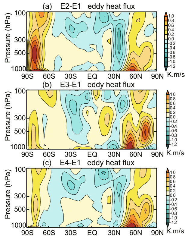
Fig. 7. The differences in annual mean eddy heat flux ( \sqrt{v'T'} ) between runs (a) E2 and E1, (b) E3 and E1, and (c) E4 and E1.
