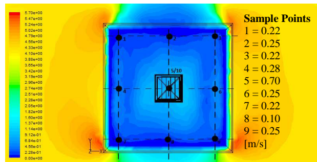
Figure 18 Contour plot of internal velocity at external velocity of 4 m/s showing the location of sample points within the microclimate (Modern wind tower).
