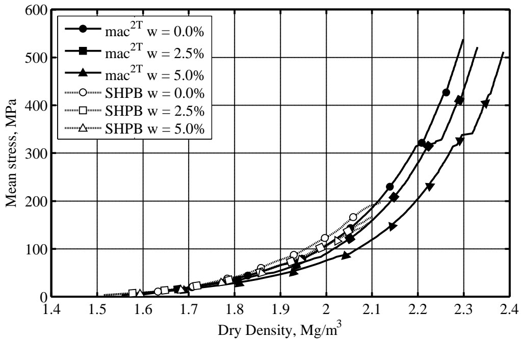
Figure 10: Mean stress–dry density data for mac 2T and SHPB tests with varying moisture content. Mean results are presented and unloading omitted for clarity.
