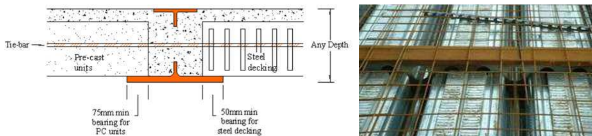
Fig. 1: Cross-section configuration of composite floor construction using asymmetric USFBs (left panel) and deep decking floor application (right panel) (ASDWestok Ltd.)
