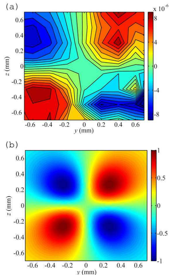
Fig. 1. (a) Contour plot showing the spatial variation of the photodiode signal measured across the y - z plane (the (110) plane) of the ZnTe crystal. The origin (0,0) corresponds to the centre of the THz beam. (b) Spatial variation of the (normalized) photodiode signal calculated using the photothermoelastic model for the same experimental conditions.
