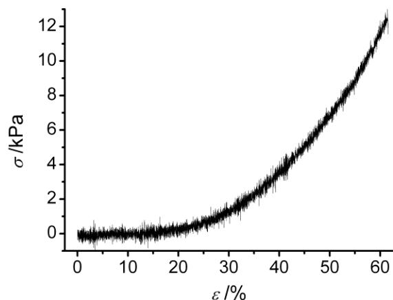
Figure 5. Compressive stress-strain plot of hydrogel Collagen-Ph1 compressed up to sample break describing a J-shaped curve, typical of native tissues. Shape recovery was observed following compression up to nearly 50%.
