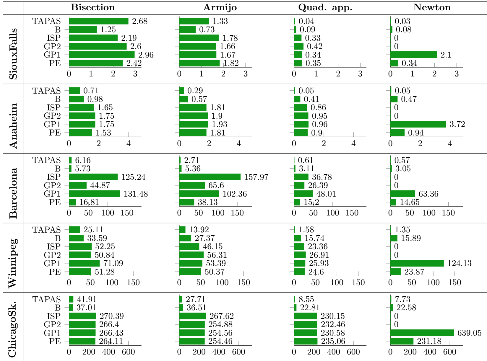
Figure 5: Test 1. CPU time, s.
