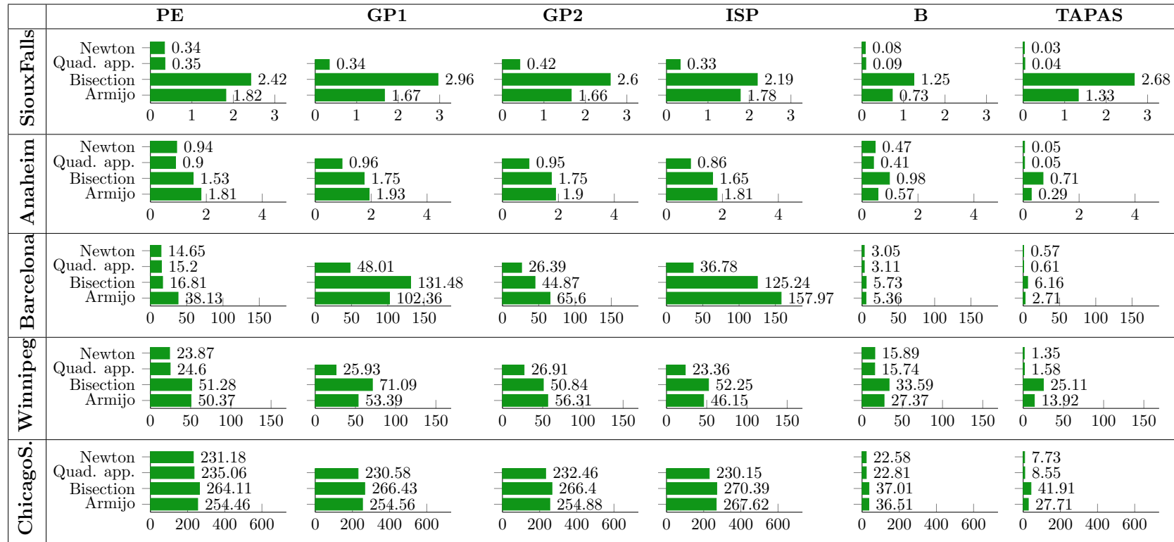
Figure 6: Test 1. CPU time, s.
