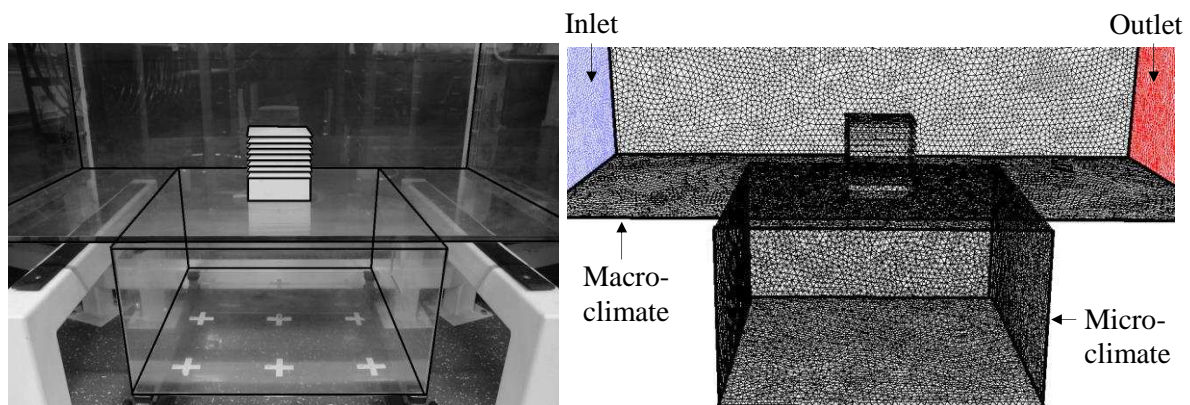
Figure 3 (a) Wind tower model inside the wind tunnel test section (b) view of the computational mesh of the wind tower model and test room
