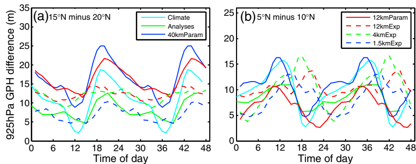
Figure 5. Mean diurnal cycle of the difference in 925 hPa geopotential height averaged over 8^{\circ}\text{W} – 6^{\circ}\text{E} and between (a) 15 and 20^{\circ}\text{N} and between (b) 5 and 10^{\circ}\text{N} .
