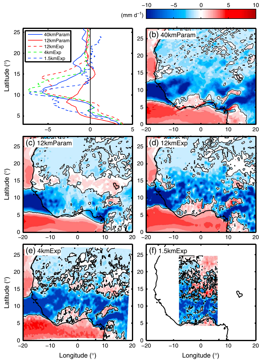
Figure 10. Forty day mean MFD integrated over whole atmospheric column. (a) Averaged between 8°W and 6°E and the x axis is MFD ( \text{mm d}^{-1} ). (b) 40kmParam, (c) 12kmParam, (d) 12kmExp, (e) 4kmExp, and (f) 1.5kmExp. The black contour is at -1 \text{ mm d}^{-1} . Due to computational limitations, MFD was only computed for 1.5kmExp within the analyses boxes marked in Figure 1 (7.5–24°N, 8°W–6°E).
