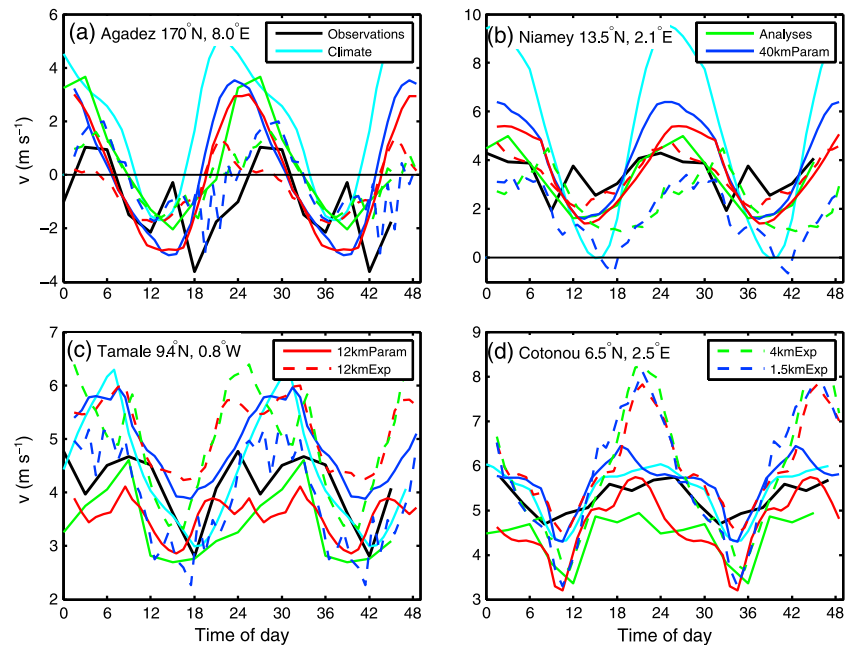
Figure 7. Mean diurnal cycle in meridional wind speeds, v , at 400 m agl from the models and observations. Note that the data for (a) the climate model was taken from 14°N, 8.0°E to allow for the fact that the entire monsoon system is too far south in this model.
