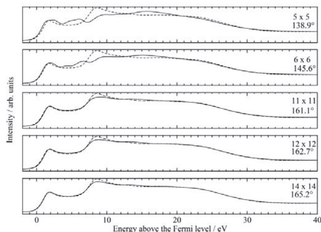
Figure 3. Predicted carbon K-edge ELNES for various labelled nanotube sizes (also labelled are angles between adjacent hexagons, which for graphene is 180^\circ ), using the CASTEP DFT code, carried out in the ground electronic state, with inequivalent positions not averaged due to similarity. The results are shown with the addition of energy-dependent final state lifetime broadening [19]. Shown on each plot is a dashed line, which is a predicted spectrum for bulk graphene (with a 25 Å vacuum to simulate the monolayer).
