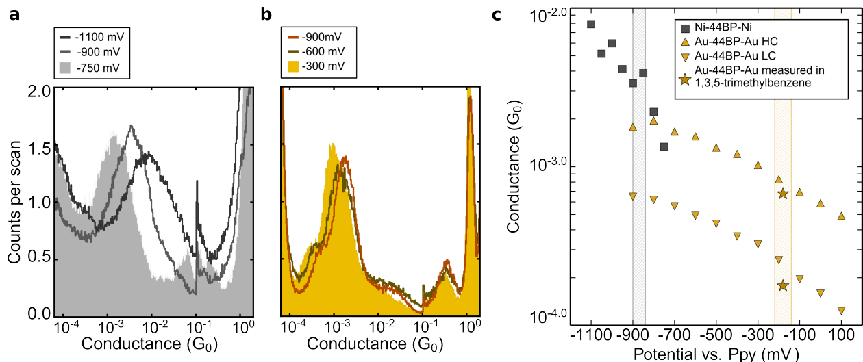
Figure 3: Conductance histograms obtained for Ni-44BP-Ni (a) and Au-44BP-Au (b) single-molecule junctions with various different potentials applied to the substrate. (c) The mean conductance values measured for Ni-44BP-Ni and Au-44BP-Au junctions under electrochemical control are plotted as a function of substrate potential. The conductance values measured for Au-44BP-Au junctions in 1,3,5-trimethylbenzene solvent are plotted at the potential of zero charge (PZC) of Au electrodes in a non-specifically adsorbing \text{HClO}_4 electrolyte, which is -0.18 V vs. the PPy scale. 31 The PZCs for Ni (-0.87 V vs. PPy 31 ) and Au electrodes in \text{HClO}_4 are indicated by the grey and gold shaded regions respectively. (PPy = +0.31 V vs. SCE)
