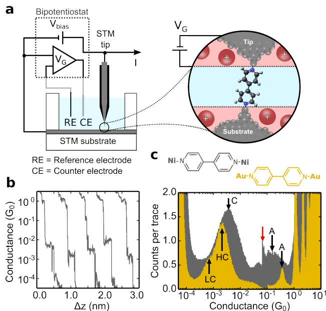
Figure 1: (a) Schematic diagram of the 4-electrode cell and cartoon of the electrochemical double layer over which the gate voltage ( V_G ) is applied. (b) Example conductance-distance traces obtained for Ni-44BP-Ni single-molecule junctions with a substrate potential of -0.9 V. \Delta z is the relative displacement of the tip which is offset laterally in each scan for clarity. (c) Logarithmically binned conductance histograms for Ni (grey) and Au (yellow) junctions generated from 1441 and 2200 scans, respectively, obtained at -0.9 V without data selection. The spike-like feature (labelled with a red arrow) is an artefact of the dual-channel pre-amplifier used for the measurements (see Supporting Information).
