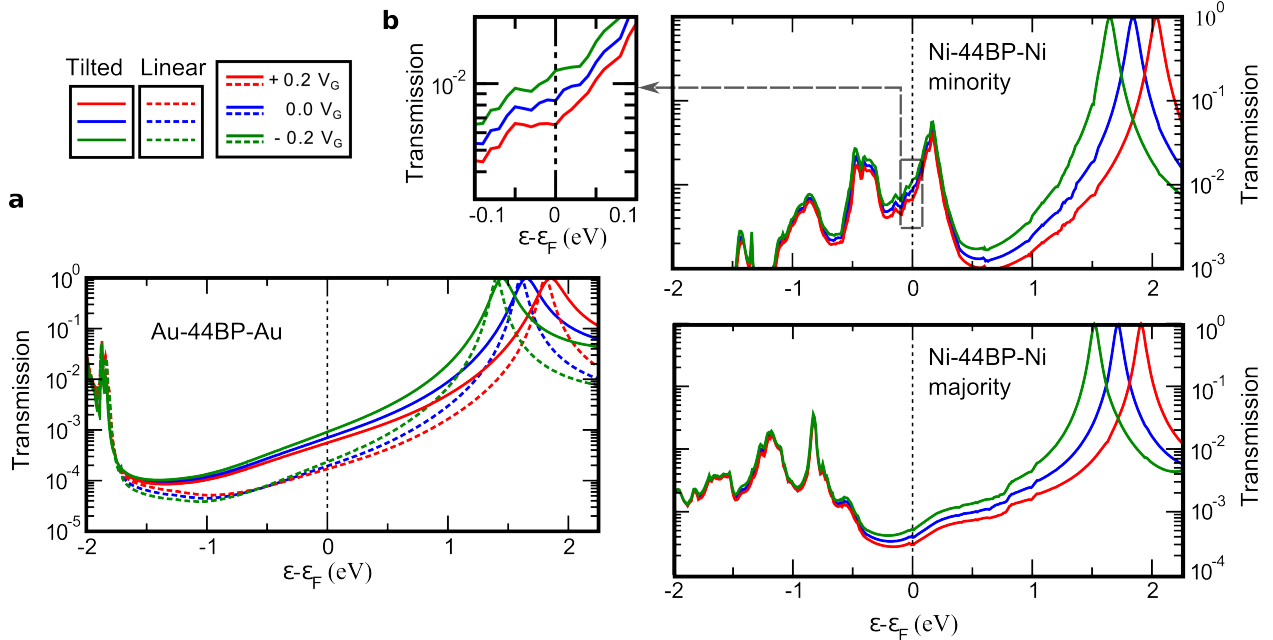
Figure 4: Transmission functions calculated at different gate voltages for (a) Au-44BP-Au junctions in the tilted configuration (solid lines), and the linear configuration (dashed lines), and (b) spin-polarized Ni-44BP-Ni junctions in the tilted configuration. The upper panel shows the Ni minority spin channel, and the lower panel shows the majority channel. The inset shows a zoomed-in area of the transmission curves around the Fermi energy for the minority channel with different gate voltages. For clarity the linear configuration is not shown but the transmission at \epsilon_F is very similar to that of the tilted configuration (See Supporting Information).
