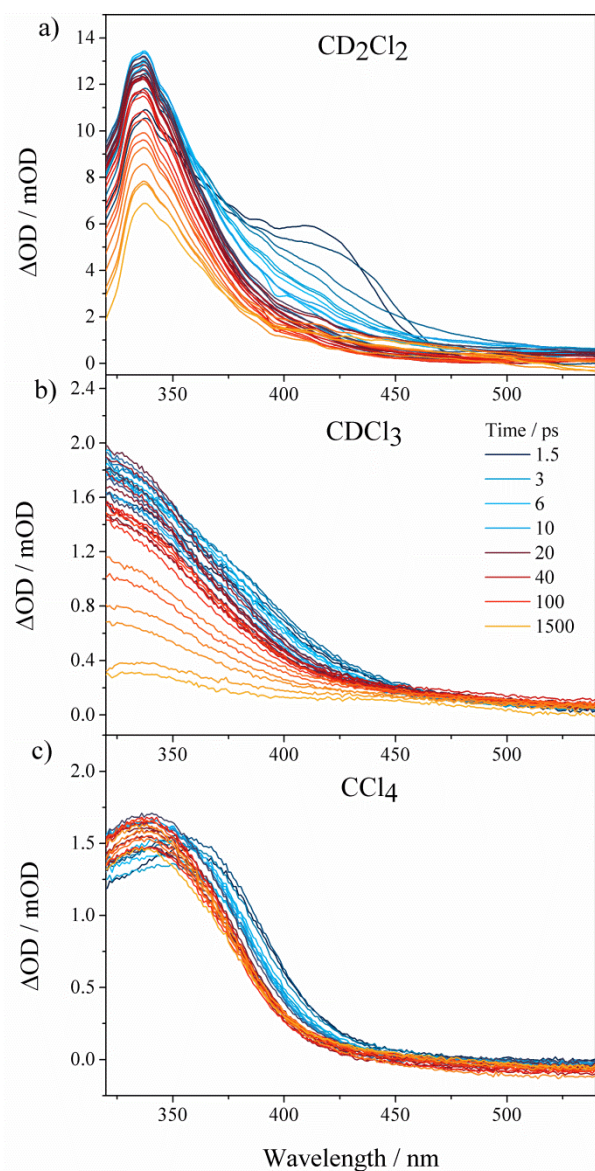
FIGURE 7. Time resolved transient absorption spectra following 266 nm photolysis of \text{XeF}_2 in a) \text{CD}_2\text{Cl}_2 , b) \text{CDCl}_3 and c) \text{CCl}_4 . The late time spectra correspond to \text{XeF}(X) absorption. The prompt broad feature in the \text{CD}_2\text{Cl}_2 data is attributed to the \text{FXe-F} complex. Absorptions caused by the 266 nm photolysis of these chlorinated solvents have been removed.
