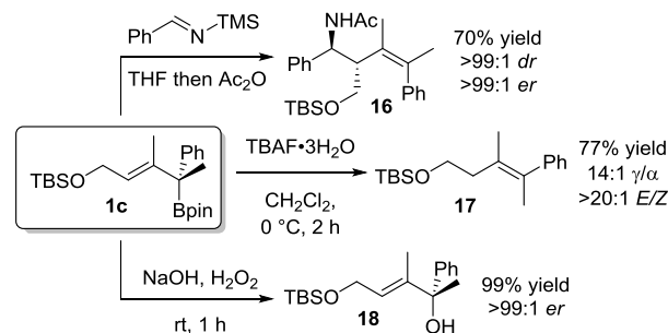
Scheme 4. Further transformations of 10 .
