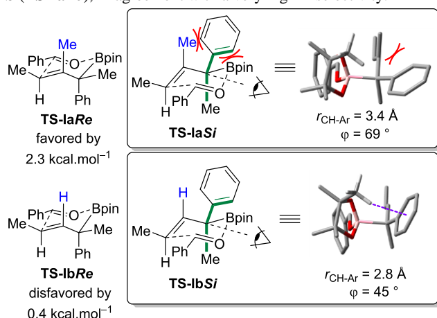
Figure 1. Calculated allylboration transition states
