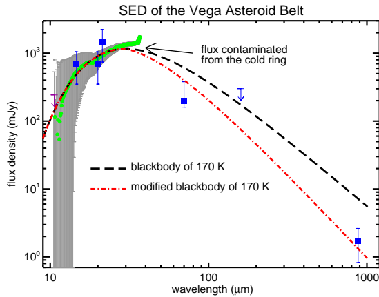
FIG. 6.— Excess SED of the inner warm component in Vega. The photospheric subtracted IRS spectrum is shown as green dots with errors (including the 2% errors from the photosphere) shown as gray area; other IR and submillimeter excess photometry are shown as blue squares. For comparison, blackbody curves of 170 K are also shown with B_\lambda as the long-dashed line and \lambda^{-0.5}B_\lambda as the dotted-dash line. The 10.6 \mu\text{m} BLINC/MMT 1\sigma upper limit is also shown.
