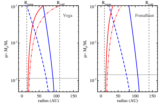
FIG. 9.— Mass-dependent chaotic zones for two equal-mass planets in the Vega (left panel (a)) and Fomalhaut (right panel (b)) systems, related to the boundaries of the inner and outer belts (shown as black, dashed, vertical lines). In both panels, the orbital radius of the inner planet is shown as red solid lines while the one of the outer planet is shown as blue solid lines. In Vega, the chaotic zone width is computed using e = 0 for the planet’s eccentricity, but for Fomalhaut we adopt e = 0.1 . The dotted-dash lines represent the outer boundary of the chaotic zone for the inner planet while the long-dashed lines represent the inner boundary of the chaotic zone for the outer planet. For two equal-mass planets, the planet-star mass ratio, \mu , has to be greater than 0.015 (0.03) for these two planets to maintain the dust-free zone in the Vega (Fomalhaut) system. The current observational upper limit for the planet mass is shown as the horizontal dotted lines.
