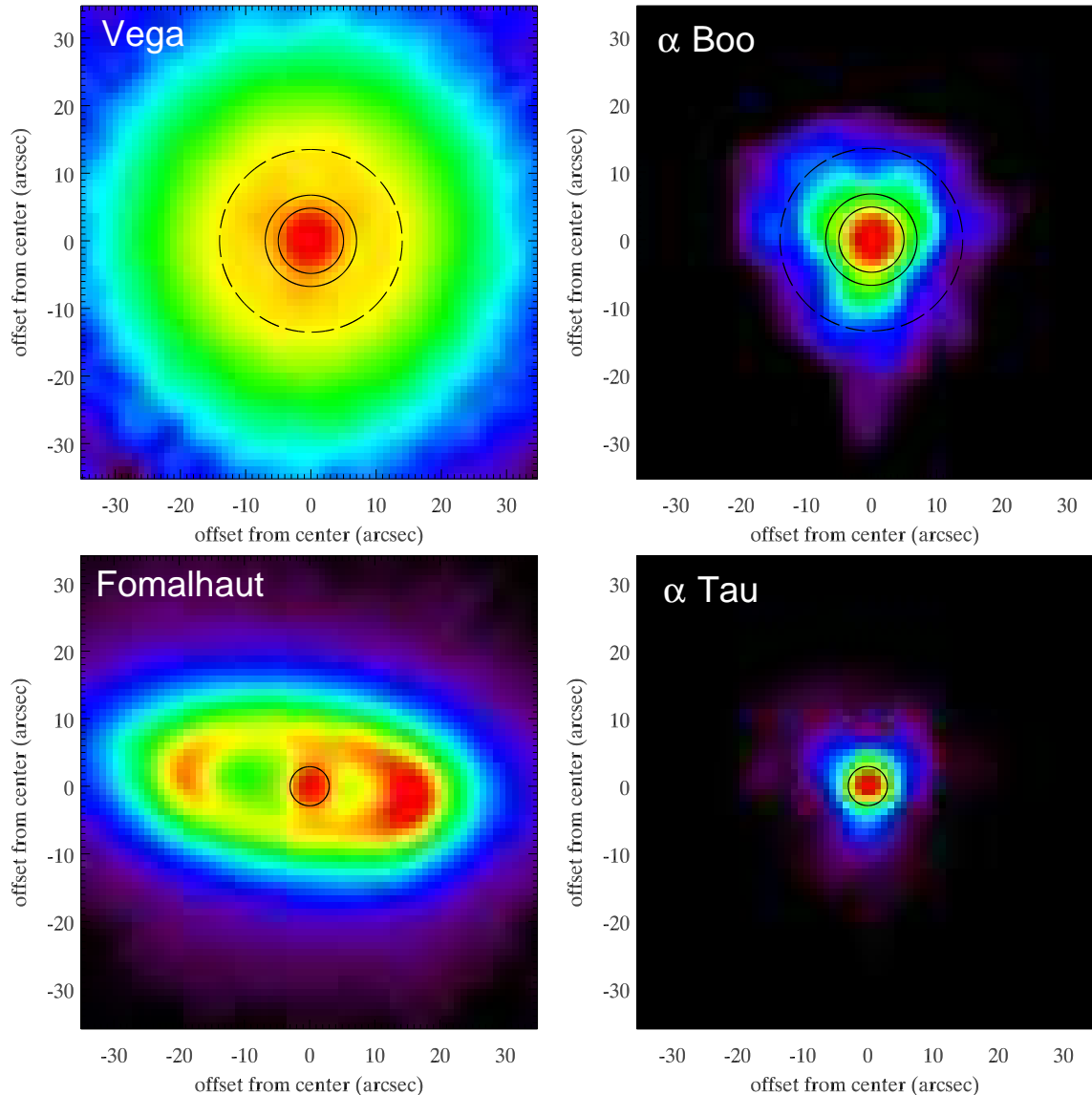
FIG. 3.— PACS 70\ \mu\text{m} images of Vega and Fomalhaut along with their reference PSF stars, \alpha\ \text{Boo} , and \alpha\ \text{Tau} . All images are shown in the same angular scale and in the PACS array orientation, i.e., the sub-structures of the PSF are in the same orientation in all four images. The dynamic range of display is from the peak value to 1% of the peak value. The color scheme is in logarithmic scale for Vega and \alpha\ \text{Boo} , but in squared root scale for Fomalhaut and \alpha\ \text{Tau} for clarity. In the Vega and \alpha\ \text{Boo} images, the two solid circles mark radii of 5'' and 7'' while the dashed circle marks a radius of 14'' (representing the cold planetesimal ring). In the Fomalhaut and \alpha\ \text{Tau} images, the solid circles mark a radius of 3'' .
