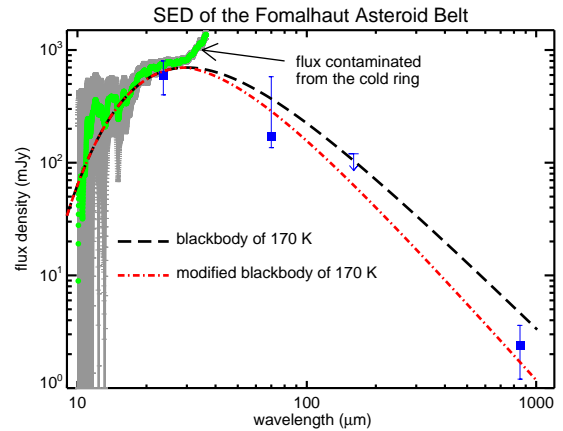
FIG. 7.— Excess SED of the inner warm component in Fomalhaut. Symbols and lines are similar to what were used in Figure 6. The upper error bar at 70 \mu\text{m} represents the (unlikely) maximum value estimated from small aperture photometry and the lower error bar is 20% lower than the estimate from PSF subtraction. Other error bars are shown as 1\text{-}\sigma . For comparison, blackbody curves of 170 K are also shown with B_\lambda as the long-dashed line and \lambda^{-0.5}B_\lambda as the dotted-dash line.
