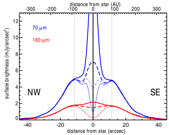
FIG. 4.— Surface brightness cuts for the Vega system. These cuts were centered at the star position and represent the mean value over a width of 5 pixels along the PA of 120^\circ (along the horizontal axis in this image). The profiles at 70\ \mu\text{m} are shown in blue color while the ones at 160\ \mu\text{m} in red. The original cuts (without PSF subtraction) are shown in thick solid lines, and the long-dashed lines represent the cuts after the subtraction of photosphere. Other thin lines represent the cuts made with different levels of subtractions (scaling of the PSF). For details see Section 3.2.
