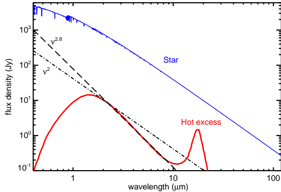
FIG. 10.— Model SED of the hot excess around Vega using nano oxide particles. Although the stellar spectrum shown on this plot (blue, thin, solid line) is the Kurucz atmospheric model (viewed pole-on), the actual heating spectrum is used the one viewed by the dust along the equator of Vega. The model spectrum (solid red line) and various power-law lines (as frequency \nu ) are normalized to 2.2 \mu\text{m} to account for the 1.29% excess at K band.
