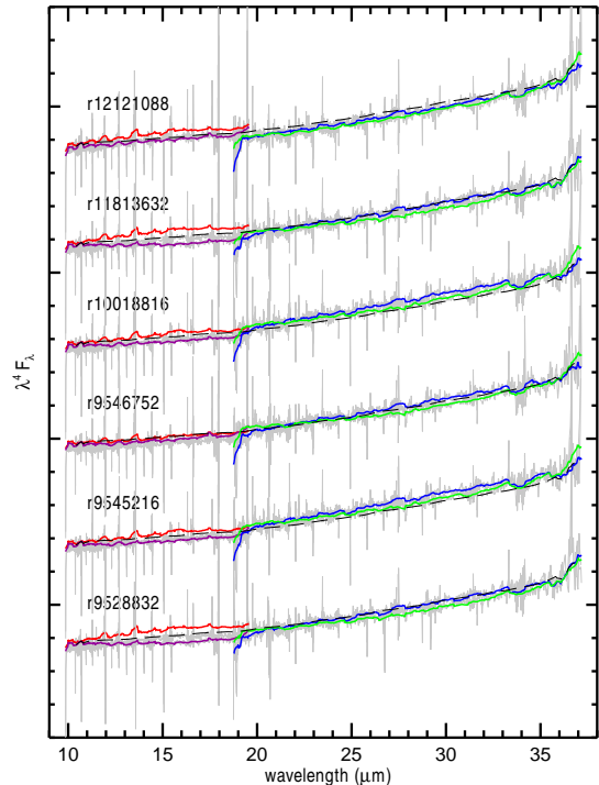
FIG. 1.— IRS spectra of Vega shown in \lambda vs. \lambda^4 F_\lambda format so that a Rayleigh-Jeans spectrum is flat. Each observation (AOR) is shifted vertically for clear viewing. The unsmoothed, unscaled extracted spectra are shown in gray lines, and the scaled, smoothed spectra are shown in colors: red and purple for SH while blue and green for LH. The final combined spectrum (black dashed line) is also shown in all six AORs for comparison.
