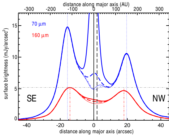
FIG. 5.— Surface brightness cuts along the major axis of the Fomalhaut system. These cuts were centered at the star position (marked as the solid vertical line) and represent the mean value over a width of 4 pixels along the minor-axis. Line styles and colors are similar to those used in Figure 4. The dotted and dotted-dash vertical lines mark the peak positions of the ansae at 70 and 160 \mu\text{m} , respectively, while the long-dashed vertical line represents the mid-point of the cold ring.
