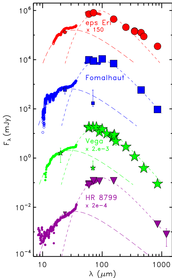
FIG. 8.— Excess SEDs for \epsilon Eri, Fomalhaut, Vega and HR 8799 where measurements are shown in various symbols with colors differentiating the objects and large size symbols being the integrated photometry while smaller ones representing spectroscopic measurements. The photometry of the warm components is also shown as the smaller symbol. The excess of each system is well represented by two (warm as long-dashed line and cold as dashed line) blackbody emissions: \epsilon Eri: 150 K and 50 K, Fomalhaut: 170 K and 50 K, Vega: 170 K and 50 K, and HR 8799: 150 K and 45 K. Note that the cold component is modeled with modified blackbody as \lambda^{-0.9} B_{\lambda} in order to fit the sub-millimeter observations.
