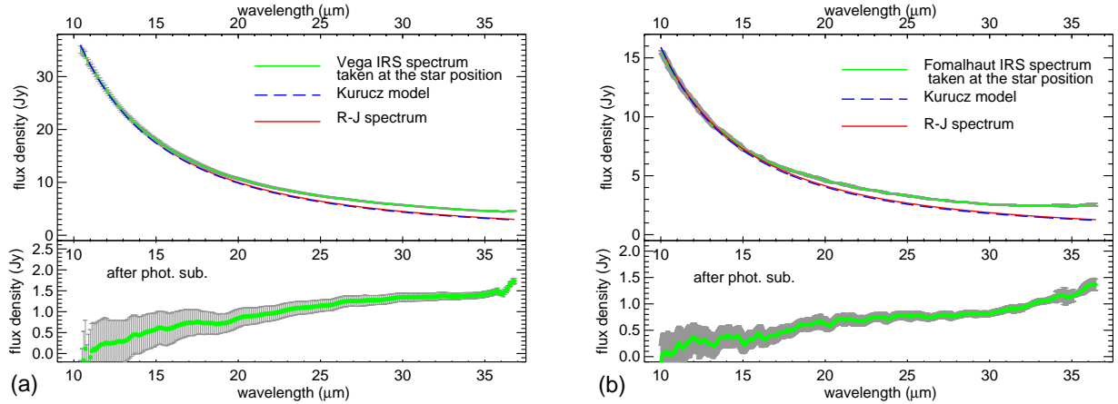
FIG. 2. — Spitzer IRS spectra centered at the star position for Vega (upper panel a) and Fomalhaut (upper panel b). For comparison, Kurucz atmospheric models (long dashed lines) and Rayleigh-Jeans spectra (solid red lines) are also shown. The excess spectra (after photospheric subtraction) are shown in the lower panels of the plots. The errors for these excess spectra include 2% uncertainty from the photospheric models.
