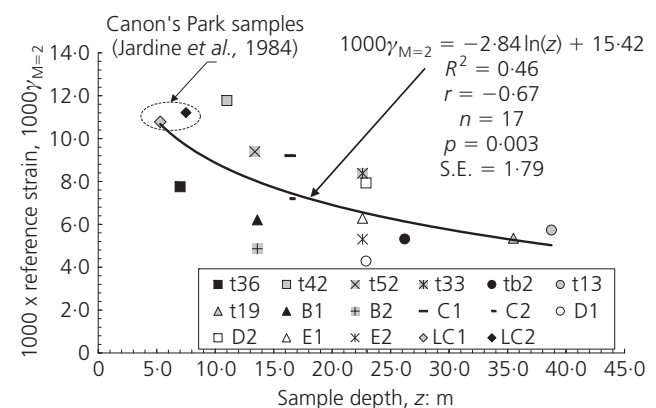
Figure 9. Mobilisation strain plotted against sample depth for three sites in London Clay (after Vardanega and Bolton, 2011b)
