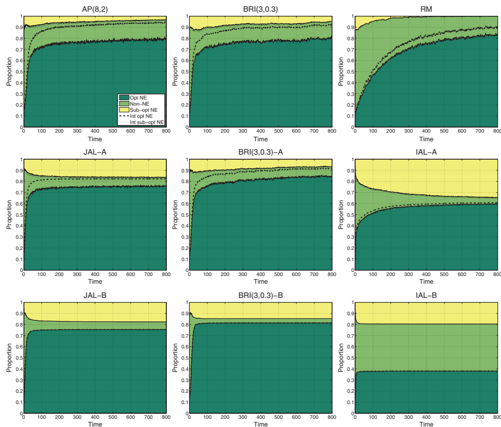
FIG. 6.2. Action proportions over time, showing the optimal, suboptimal, and non-Nash equilibrium play and intended play (without sampling) superimposed.
