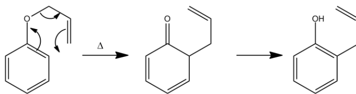
Scheme 2 – Thermal Claisen rearrangement of allyl phenyl ether.
