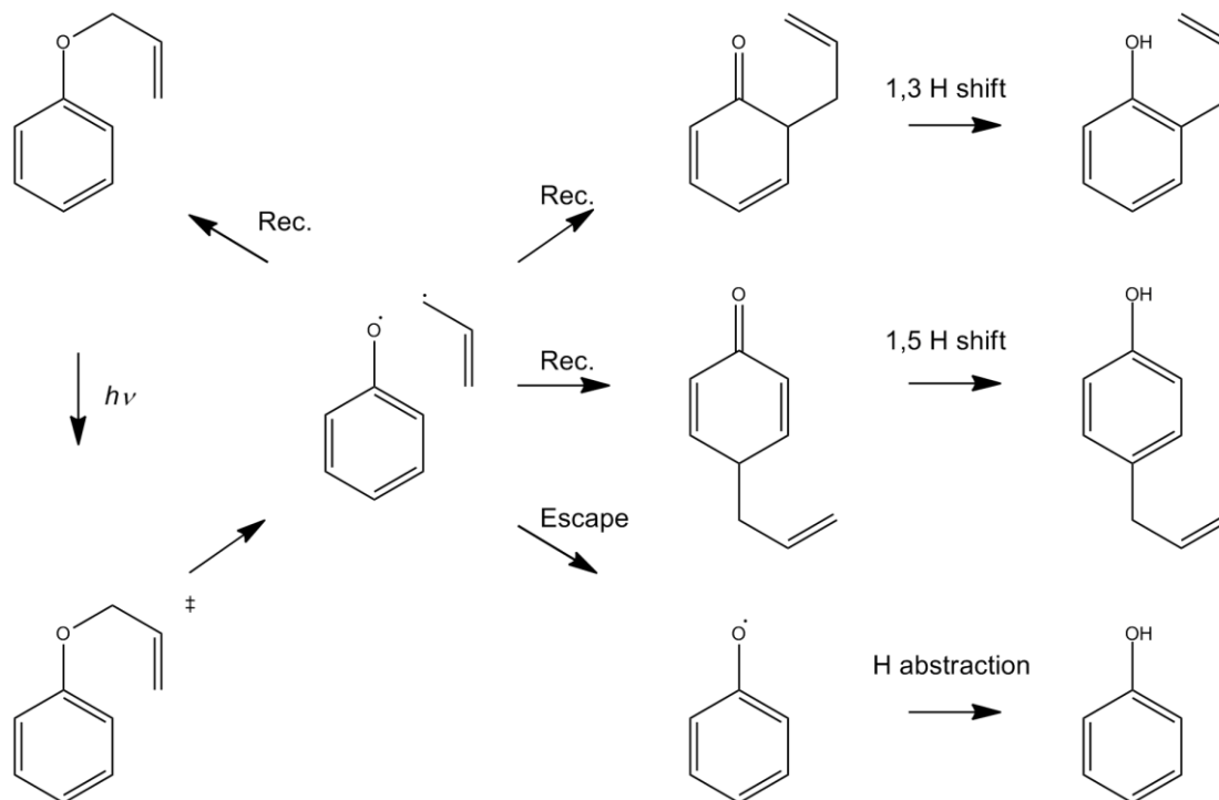
Scheme 3 – Photo-Claisen rearrangement of allyl phenyl ether.
