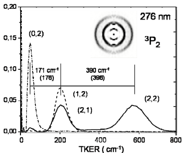
Figure 4. Inverted S(^3P_2) image (see Fig. 3 caption for details) and Total Kinetic Energy Release (TKER) distributions for S(^3P_J) atoms, J = 2, 1, 0 , from the photodissociation of S_2 at 276 nm. The labels (i, j) indicate S(^3P_i) + S(^3P_j) products, with i referring to the measured atom and j to the co-fragment. The solid, dashed, and dash-dot lines are for S(^3P_J) J = 2, 1 , and 0 detection, respectively. The measured TKER spacing between the peaks at 171 \text{ cm}^{-1} and 390 \text{ cm}^{-1} agree well with the known S(^3P_J) J = 2-1 , and 1-0 spin-orbit level separations of 176 \text{ cm}^{-1} and 396 \text{ cm}^{-1} . The (2, 2) peak is wider than (2, 1) due to the limited pixel resolution of this small image (both rings are one pixel wide at their half-maximum in velocity space, in KER the width increases as velocity squared).
