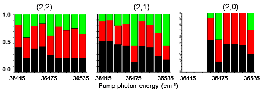
Figure 9. Relative populations of |m_j| levels for the J=2 atoms formed via (2,2), (2,1), and (2,0) photofragmentation channels of S_2 : |m_j|=2 green, |m_j|=1 red, and |m_j|=0 black. Data are presented at several different dissociation energies that coincide with the region of S_2 absorption in the vicinity of the B(v'=12) - X band.
