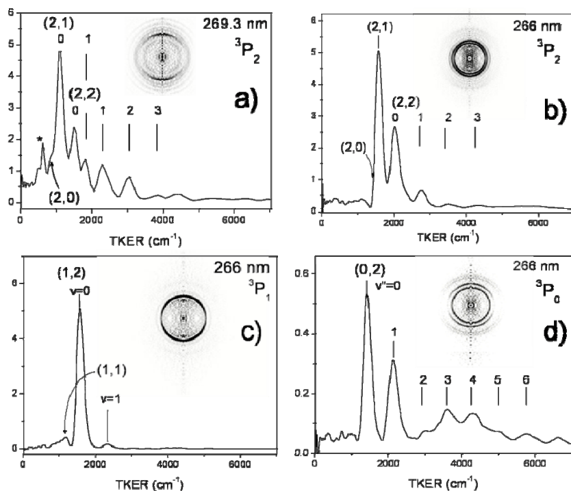
Figure 6. Inverted images and TKER distributions for S(^3P_J) following photodissociation of S_2 at 269.3 and 266 nm. Panels (a) and (b) are for S(^3P_2) detection, at respective photodissociation wavelengths of 269.3 and 266 nm; panels (c) and (d) show data obtained for S(^3P_1) and S(^3P_0) detection, and a photodissociation wavelength of 266 nm. The combs of vertical lines in the panels indicate features in the TKER distributions that are assigned to photodissociation of S_2(v'') with v'' = 0 and above.
