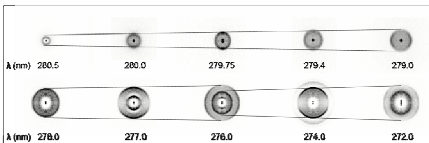
Figure 3. Raw S^3P_2 ) velocity map images from S_2 photodissociation at the indicated wavelengths. The linear photolysis laser polarization is along the vertical axis. Darker regions correspond to higher signal. Straight lines used to connect the same channel in different images are only to help guide the eye, as the energy spacing is irregular.
