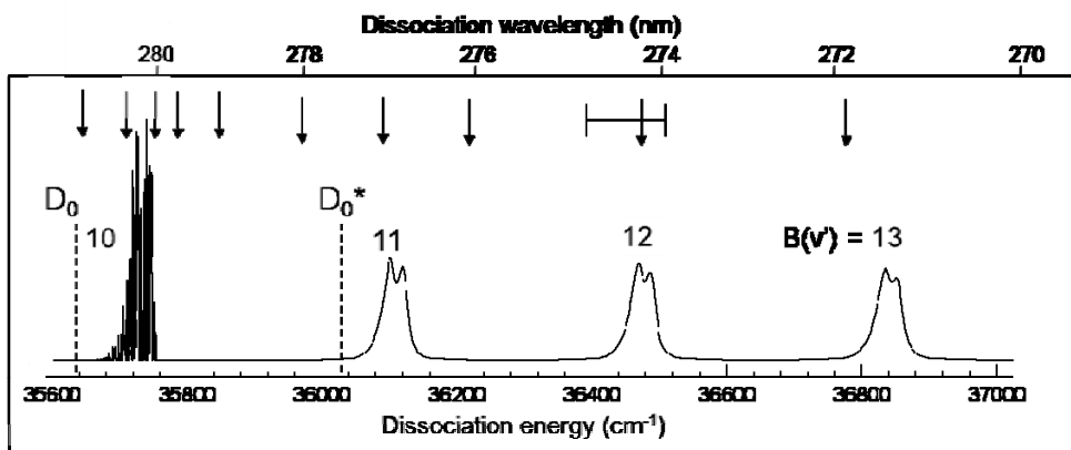
Figure 2. Simulation of the UV absorption spectrum of the B-X transition at a temperature of 50 K from the constants and linewidths given by Wheeler et al. 15 using the PGOPHER program. 32 Velocity map images were obtained for photolysis wavelengths indicated by the position of the vertical arrows. The new value of D_0 obtained in this study is shown by a dashed vertical line, and the second dashed line, labelled by D_0^* shows the onset for dissociation to the (2,1) limit.
