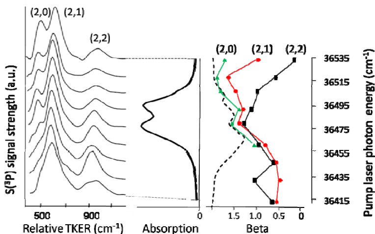
Figure 7. a) S(^3P_2) atom TKER distributions, b) simulated S_2 B(v'=12) absorption spectrum at 50 K, and c) recoil velocity anisotropy parameters, \beta (right) for S_2 photodissociation in the region from 36415 cm -1 to 36535 cm -1 . The dashed line in the right-hand panel c) is the result of the beta of nu simulation program 34 : (see text).
