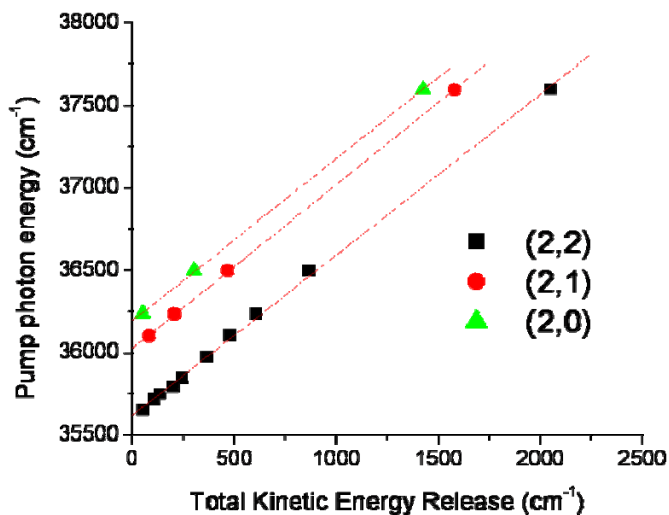
Figure 5. Plots of photolysis laser photon wavenumber against photofragment TKER for S(^3P_J) products of S_2 photodissociation at wavelengths from 266 – 281 nm. Extrapolation to TKER = 0 is used to determine the S_2 bond dissociation energy. Detection of S(^3P_J) with J = 2, 1 and 0 is indicated by squares, circles, and triangles, respectively, and the co-fragment is S(^3P_2) .
