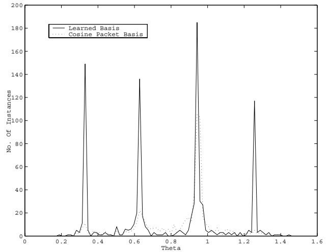
Fig. 2. Histogram plot of the values of \theta obtained from the dual matching pursuit using both a cosine packet and a learned reduced basis. The range 0 to \pi/2 is divided into 100 bins.
