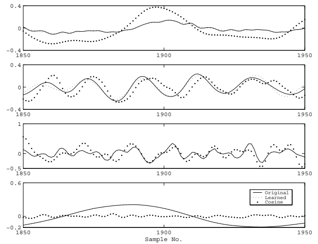
Fig. 3. Waveform plots of 100 samples from sources 1 to 4 (top to bottom) (solid line) and inferred sources using the dual matching pursuit using the cosine packet basis ( \bullet ) and the learned reduced basis ( \dots ).
