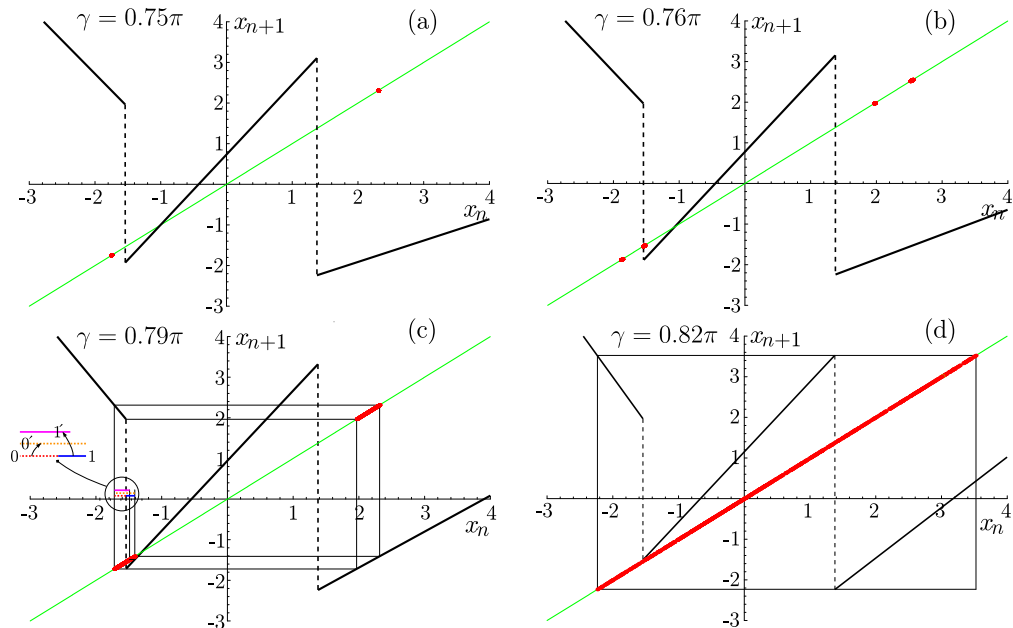
Figure 8: Return maps on the switching line \mathcal{K}_0 as a function of the projection angle \gamma . A period two attractor (a) undergoes a period doubling bifurcation (b), which induces a chaotic motion (c). The chaotic attractor shrinks to a point and a new, larger attractor arises (d).
