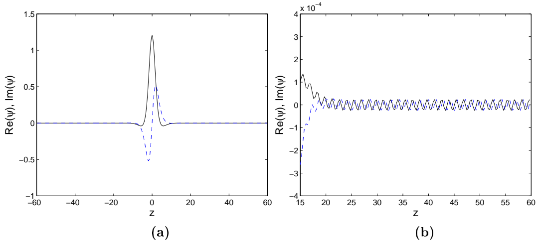
Figure 7: Results obtained using the Powell hybrid method with \varepsilon = 1, c = 0.7, \Lambda = 0.5, L = 120 . Solid line indicates \text{Re}(\psi) , dashed line shows \text{Im}(\psi) . (a) Shape of full solution. (b) Magnification of the tail exhibiting oscillations.
