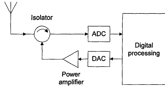
Figure 2: "Ideal" software-defined radio architecture
