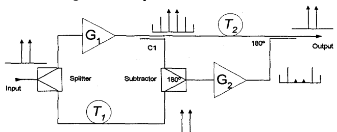
Figure 3: Feedforward linearisation architecture
