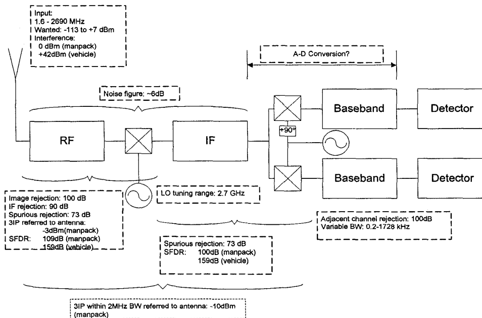
Figure 1: Outline specification for future military multi-role radio
