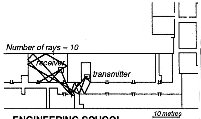
ENGINEERING SCHOOL Single location raytrace rms Delay Spread = 32 nS FIGURE 3
