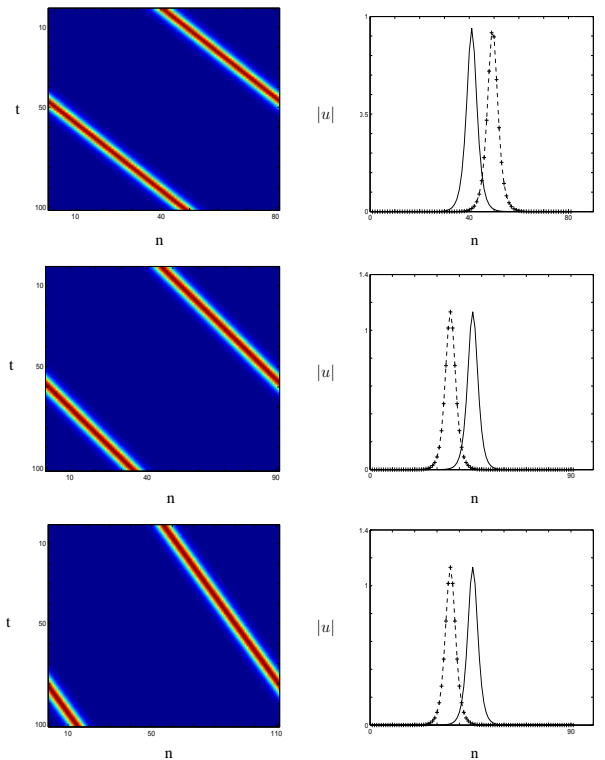
FIG. 4: (Color Online) Three examples of direct integration of the solution of branch I with \varepsilon = 0.911396 , c = 0.894153 (top panels), branch II with \varepsilon = 1.11714 , c = 0.81 (middle panels) and branch III with \varepsilon = 1.34529 , c = 0.7 (bottom panels). The space time contour plot of the solution modulus (left panels), and the modulus before (solid) and after (dashed) the solution has moved by 100 nodes (right panels) are shown.
