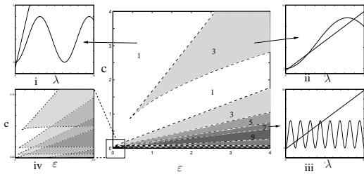
FIG. 2: Intersections of the single and double root conditions (see text) for \Lambda = 0.5 and varying c and \varepsilon . The shaded area shows where there is more than one branch of linear waves. Values indicate the number of roots of (4). Subplots show left and right hand sides of (4) for (\varepsilon, c) = (1, 3) , one root (i), (3, 3) , three roots (ii) and (3.5, 0.6) , seven roots (iii). (iv) displays the overlapping of the bands for small \varepsilon and c , only the first six bands have been shown.
