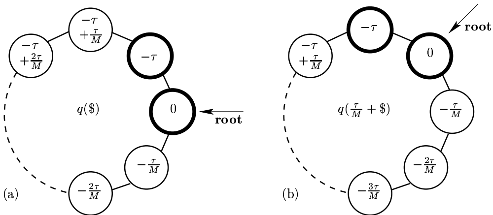
FIG. 2 One Euler integration step applied to the circular list representing a point of a DDE. The delay interval is discretized into M + 1 elements, with \$ standing for the labels of the list elements. Before the integration step root points to q(0) (a), and after the integration step root points to q(\frac{\tau}{M}) , which can be achieved by simply overwriting q(-\tau) and moving root (b). Only the two boldfaced list elements close to root are needed for one Euler step.
