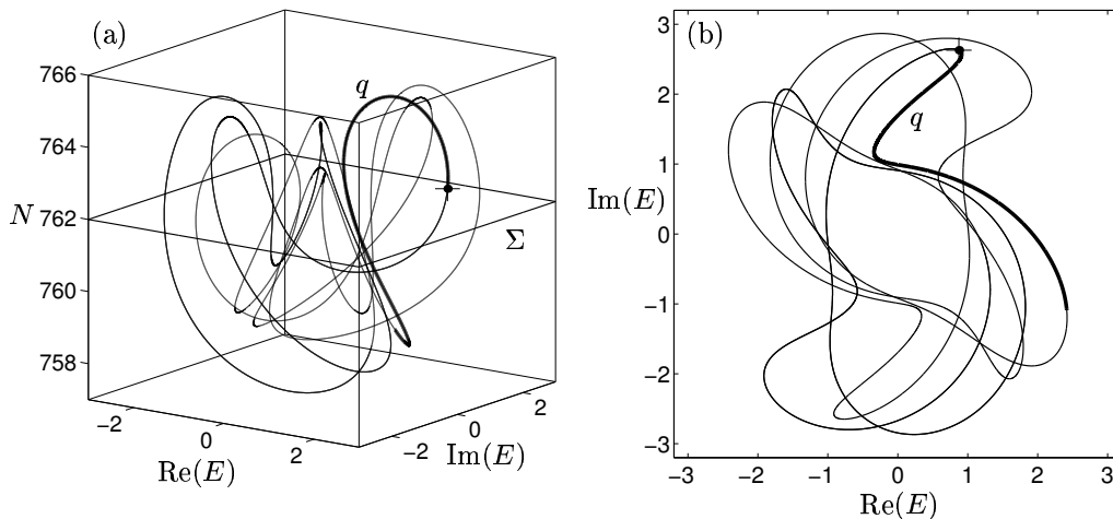
FIG. 4 A periodic orbit of the DDE and a periodic point q of the Poincaré map P (boldface), shown in (E, N) -space (a) and in the E -plane (b) for the PCF laser from (10).
