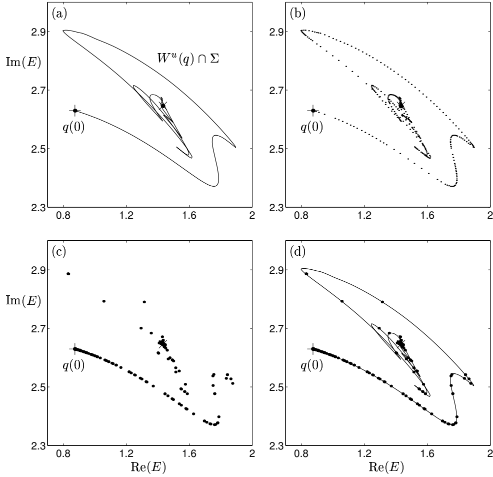
FIG. 9 The trace of one branch of the unstable manifold of the saddle-point (+), which spirals into an attractor ( \times ). Shown is the branch computed by our algorithm (a), the distribution of points along this branch (b), and the branch computed by 'naive' fundamental domain iteration (c). Part (d) shows that all points of (c) lie exactly on the computed branch from (a). This branch is for \kappa\mathcal{T} = 2.500 and it is one of the branches in Fig. 10.
