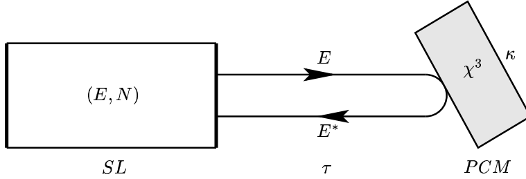
FIG. 7 Sketch of a semiconductor laser with phase-conjugate feedback.
