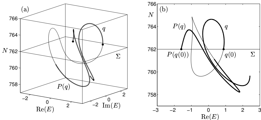
FIG. 3 The Poincaré map P takes a point q with q(0) \in \Sigma to the point P(q) with P(q(0)) \in \Sigma , which is shown in (E, N) -space (a) and in the (\text{Re}(E), N) -plane (b) for the PCF laser from (10).
