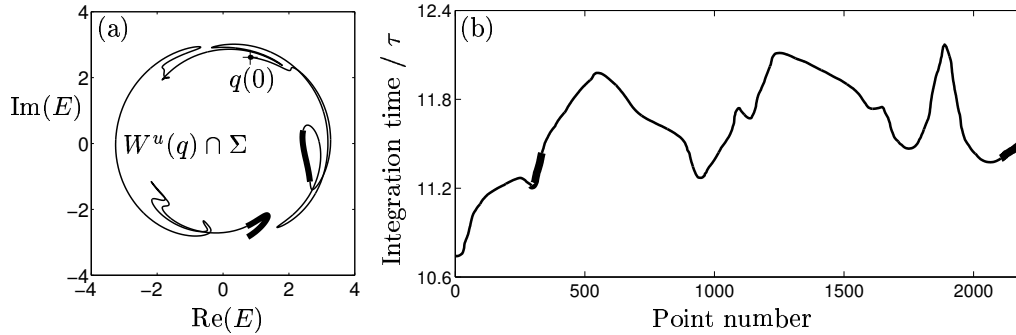
FIG. 15 Trace of a single branch of the unstable manifold for \kappa\tau = 2.550 (a) covering a large area. Boldfaced sections indicate where the Poincaré map is the 18th return to \Sigma , instead of the 20th return. Nevertheless, the integration time for each point along the branch is a continuous function (b).
