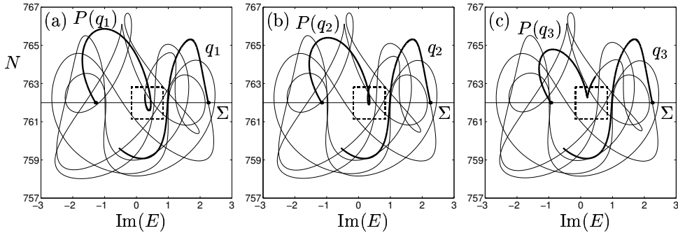
FIG. 14 Image P(q_i) and connecting trajectory shown in projection onto the (\text{Im}(E), N) -plane of three points q_1, q_2, q_3 on the branch of the unstable manifold for \kappa\tau = 2.550 shown in Fig. 15. There is a tangency in the box indicated (b), and this changes the Poincaré map from being the 20th (a) to being the 18th (c) return to \Sigma .
