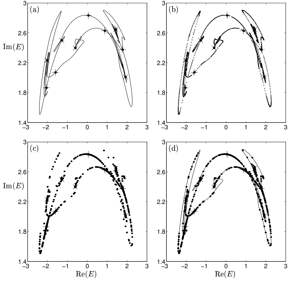
FIG. 10 The traces of all branches in \Sigma emanating from both sides of the five saddle-points (+) converging to five attractors ( \times ) for \kappa\tau = 2.500 . Panels (a)-(d) illustrate the performance of our algorithm as in Fig. 9.
