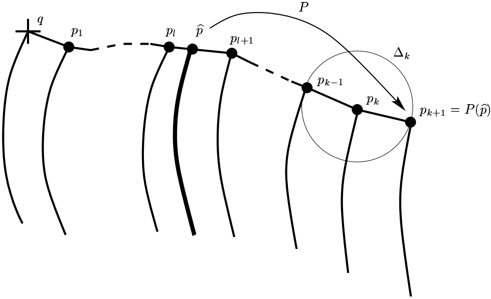
FIG. 6 Sketch of the algorithm. The new point p_{k+1} lies at distance \Delta_k from p_k , and it is found as the image of an interpolated point \hat{p} on the part of W^u(x_0) that was already computed. To indicate that we are dealing with a DDE we sketch this situation in projection onto X : the headpoint of each point lies in the section \Sigma .
