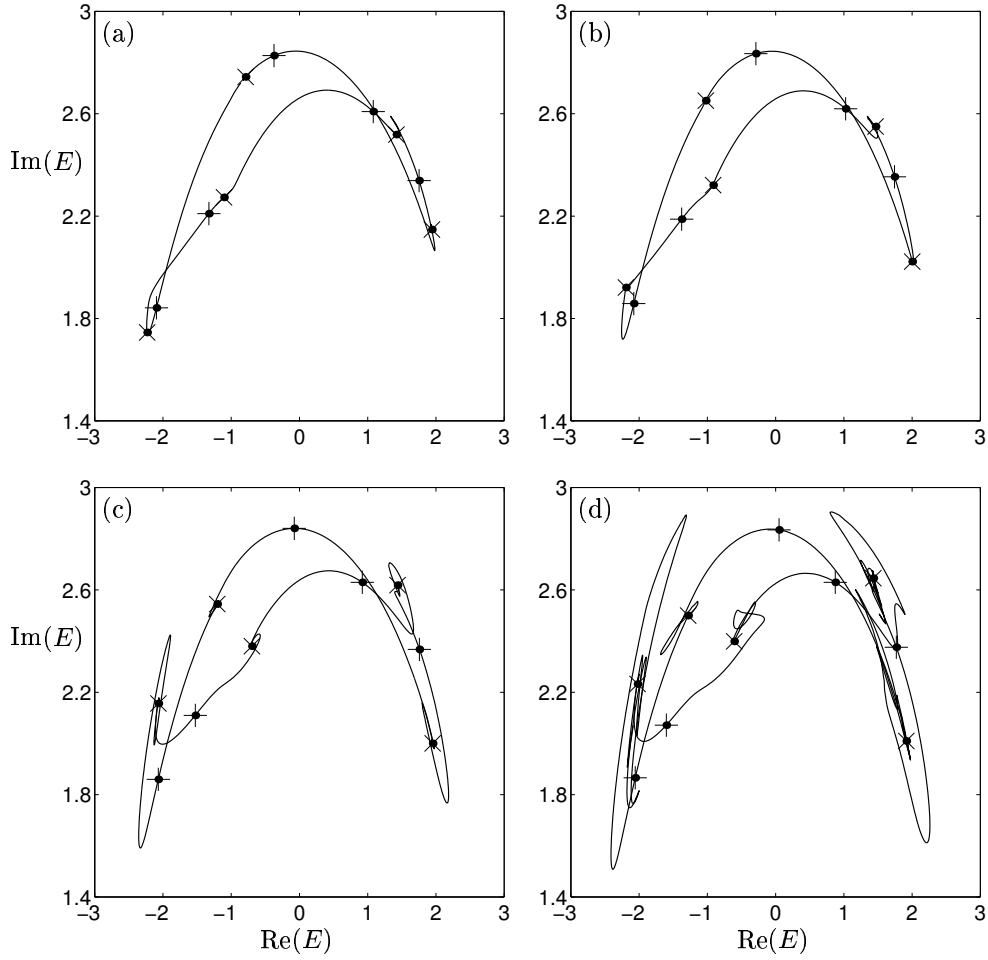
FIG. 12 As \kappa\tau is increased, the smooth torus at \kappa\tau = 2.445 (a) loses its smoothness at \kappa\tau = 2.450 (b). As \kappa\tau is increased further through \kappa\tau = 2.480 (c) and \kappa\tau = 2.500 (d), the torus becomes increasingly folded and stretched.
