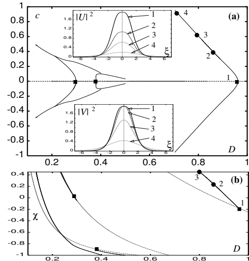
FIG. 1. The solution branches of the quiescent and moving (dotted and solid lines) embedded solitons in the case \sigma = 0 ; squares show bifurcations, circles label points. (a) The velocity vs. the effective dispersion coefficient D . The insets show typical examples of the solutions on the first branch (note the asymmetry between U and V ). (b) The effective frequency \chi vs. D .
