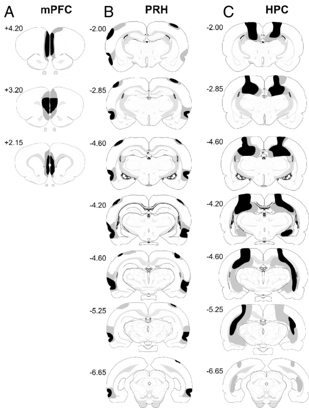
Figure 2. Diagrammatic reconstructions showing the cases with the largest (gray) and smallest (black) lesions in the mPFC ( A ), PRH ( B ), and HPC ( C ) groups. The numbers correspond to the approximate position relative to bregma (Swanson, 1998).
