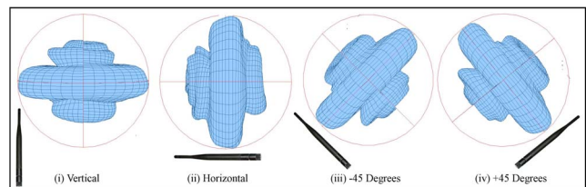
Figure 6. Antenna radiation patterns at diff. orientations (polarizations)
