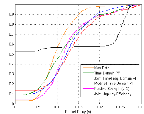
Figure 8: VoIP packet delay distributions
