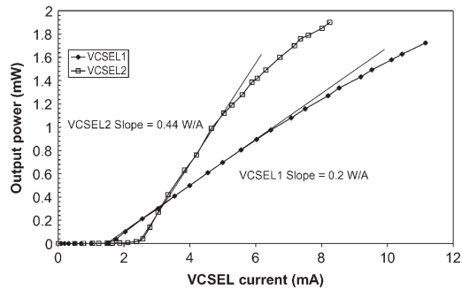
Fig. 2. L - I curves for VCSEL 1 and VCSEL 2.
