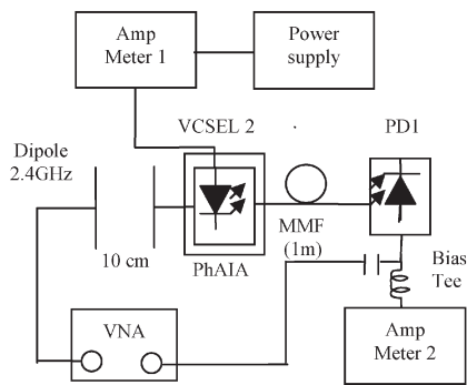
Fig. 19. S_{21} measurement diagram of VCSEL-PhAIA.
