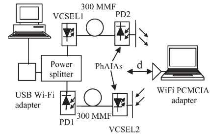
Fig. 1. System configuration.
