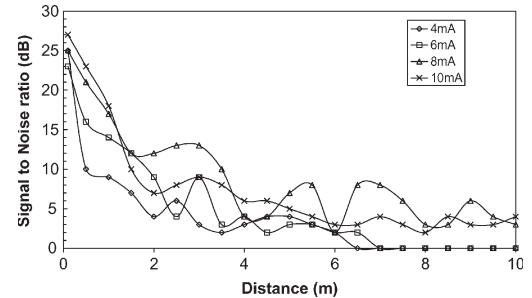
Fig. 25. SNR versus distance at different VCSEL-1 bias current.
