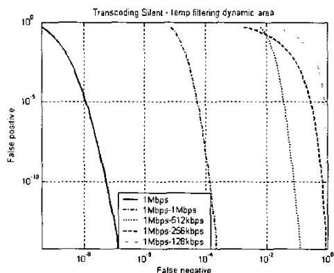
Figure 1: ROC of Silent test sequence. W extraction with temporal filtering. Watermarked sequence encoded at 1Mbps and subsequently re-encoded at 1Mbps , 512kbps , 256kbps and 128kbps
