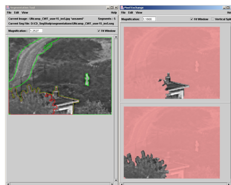
Figure 2: Segmentation Tool
