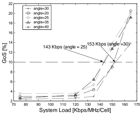
Figure 5: Spectrum efficiency for different sector orientation
