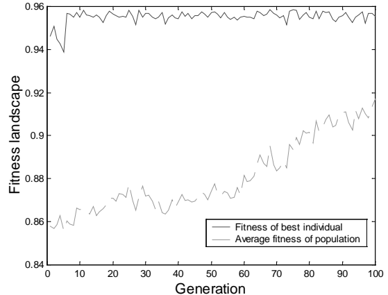
Figure 4: Fitness landscape for a deployment of 55 users (15 Kbps voice service)
