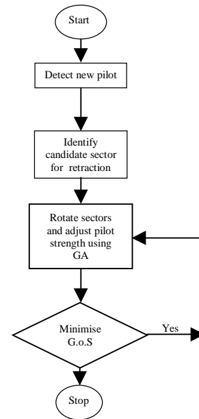
Figure 3: Coverage reconfiguration algorithm
