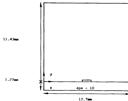
Fig. 2. Microstrip cross section.
