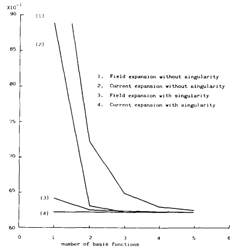
Fig. 1. Convergence with various basis functions.
