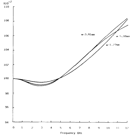
Fig. 7. Normalized characteristic impedance of microstrip. a = 12.7 mm; d = 1.27 mm; h = 10.43 mm; \epsilon_p = 8.875 .
