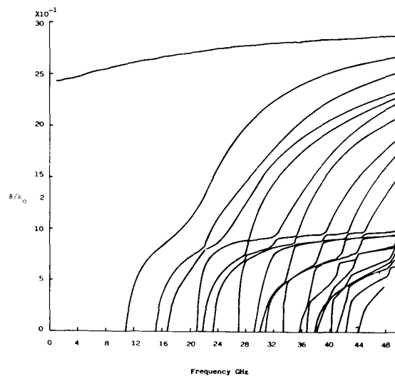
Fig. 3. Higher order modes of microstrip. a = 12.7 mm; d = 1.27 mm; h = 10.43 mm; w = 1.27 mm; \epsilon_p = 8.875 .
