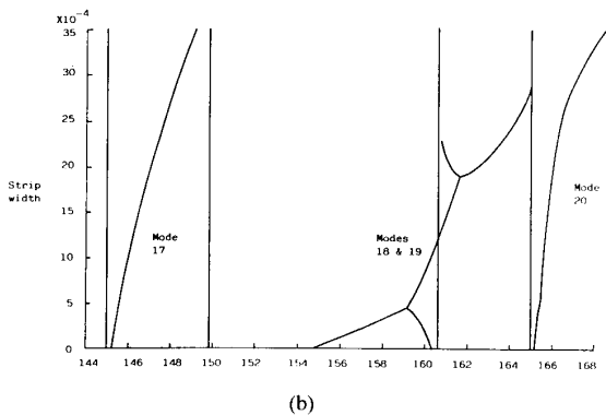
Fig. 5. (a) Effective permittivity (imag.) (\beta/k_0)^2 . (b) Effective permittivity (real) (\beta/k_0)^2 .
