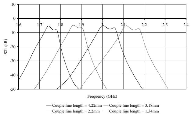
Figure 8 Measured S_{21} versus frequency for the 4 filters.
