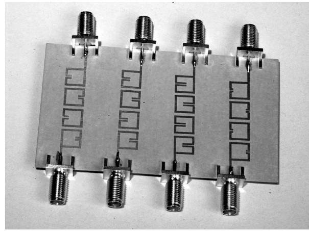
Figure 7 Prototype filters
