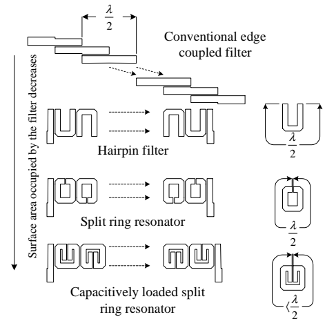
Figure 2 Evolution of the slow wave filter.
