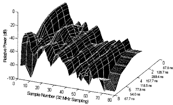
Figure 5: 'Finite Bandwidth' Profile Variation
