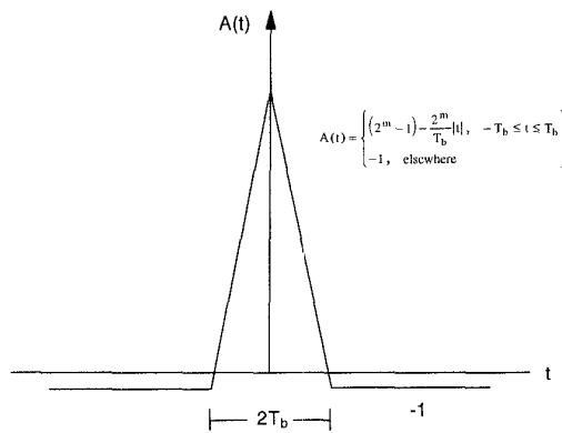
Figure 2: PN Sequence Autocorrelation
